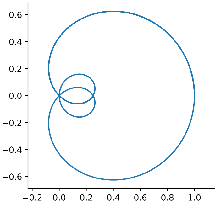
Freeth's Nephroid
