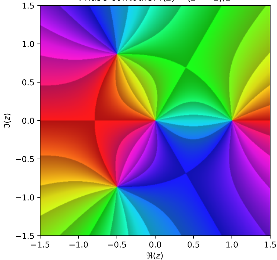
Phase contours: f(z) = (z^3 - 1)/z
