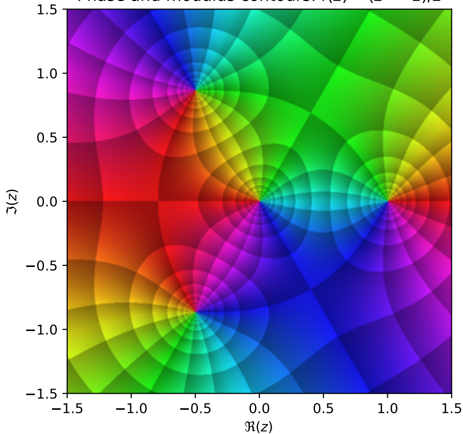
Phase and modulus contours: f(z) = (z^3 - 1)/z
