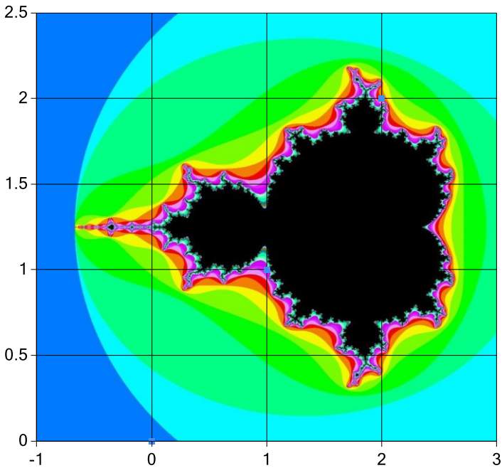
Mandelbrot set
