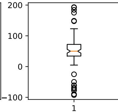
notched plot
