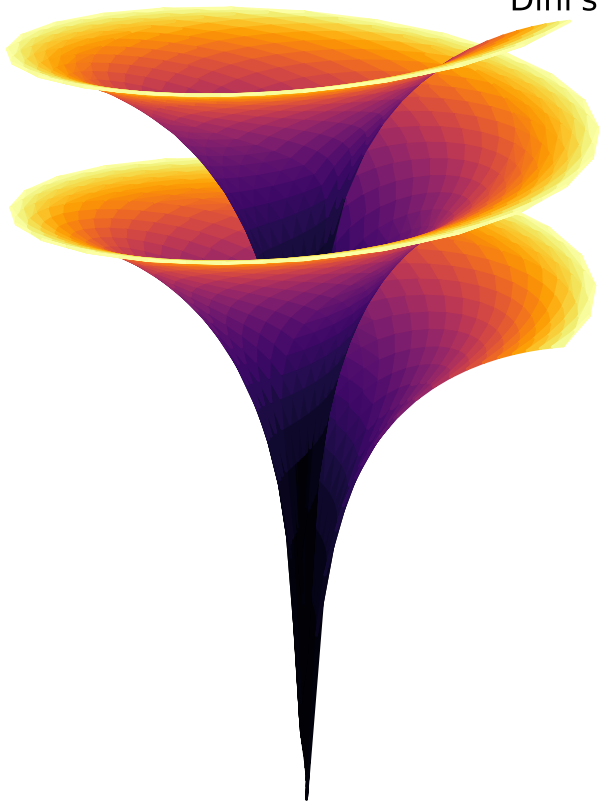
Dini's Surface
