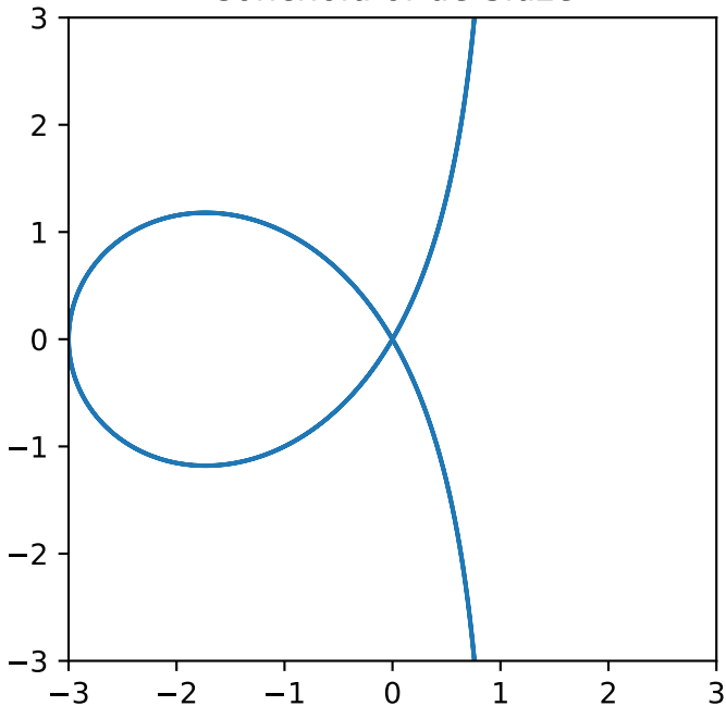
Conchoid of de Sluze
