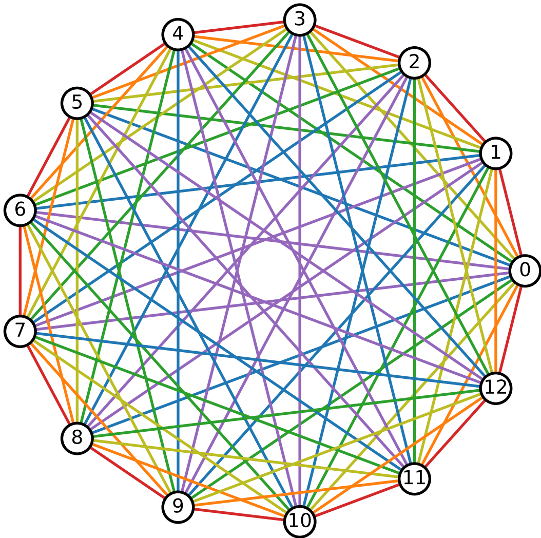
Rainbow_Coloring
