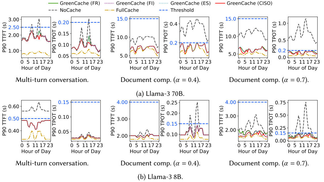
Fig. 13. SLO attainment timelines of LLM tasks.
