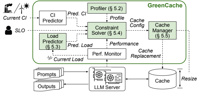
Fig. 10. System overview of GreenCache. Components in green are newly designed by this work.
