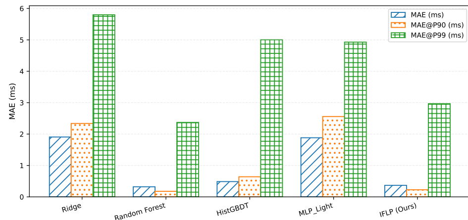
Figure 12. Prediction accuracy of candidate latency predictors. We compare MAE, P90 MAE, and P99 MAE across alternative models.
