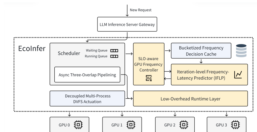
Figure 5. System overview of EcoInfer. EcoInfer is integrated into the LLM serving engine as a lightweight iteration-level DVFS control layer.
