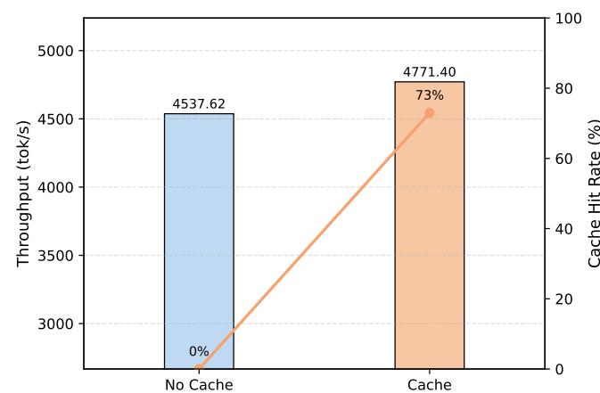
Figure 14. Effectiveness of the bucketized frequency-decision cache. Bars denote throughput, and the solid line denotes cache hit rate. The cache improves throughput while achieving a high decision-reuse rate over time.
