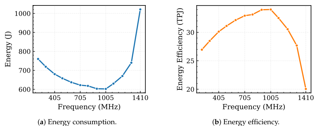
Figure 2. Energy consumption and efficiency together reveal an energy sweet spot in LLM inference under GPU frequency scaling. (a) Energy consumption exhibits a U-shaped trend across GPU frequencies. (b) Energy efficiency, measured in TPJ, shows an inverted-U trend, indicating that the most energy-efficient operating point lies at an intermediate frequency rather than at either extreme. Results are obtained by serving Qwen3-8B [30] on an A100-80G using vLLM [15].
