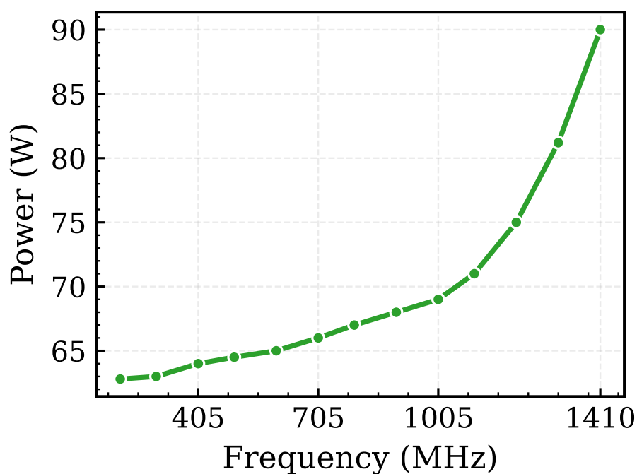
Figure 1. Relationship between GPU core frequency and power consumption under DVFS. GPU power increases monotonically with frequency and can be well approximated by a quadratic function, consistent with Equation (1).
