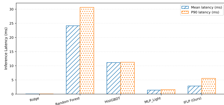
Figure 13. Inference latency of candidate prediction models. We report the mean and P90 inference latencies. Low online predictor cost is essential for practical iteration-level DVFS.
