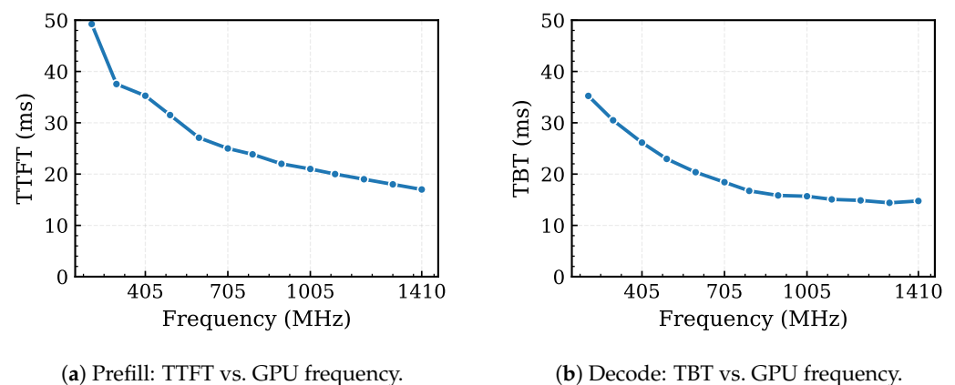
Figure 3. Latency sensitivity to GPU frequency scaling. (a) Prefill-phase TTFT increases sharply with frequency reduction. (b) Decode-phase TBT remains relatively stable even under aggressive frequency scaling, particularly when the GPU frequency is above 705 MHz.
