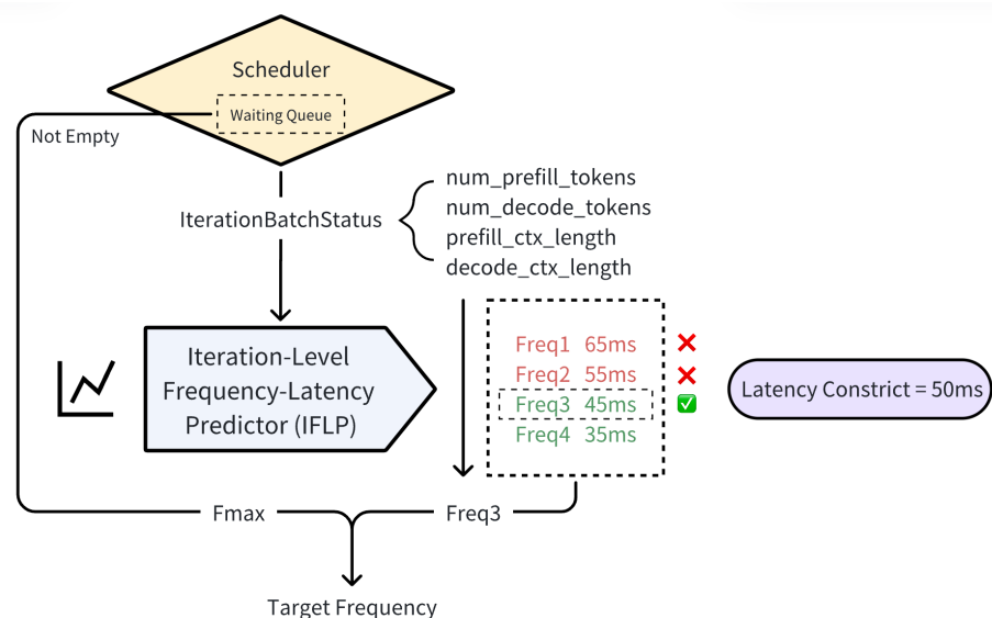
Figure 6. Frequency selection logic of the SLO-Aware GPU Frequency Controller.
