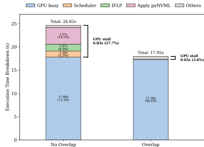
Figure 15. End-to-end execution-time breakdown of EcoInfer with the frequency-decision cache disabled, showing how scheduler, IFLP-predictor, pyNVML actuation, and GPU busy time compose the total wall-clock time. No Overlap executes all CPU-side stages synchronously before GPU forward progress, exposing 27.7% of total time as GPU stall. Overlap pipelines next-iteration scheduling and prediction with current-iteration GPU execution and decouples DVFS actuation into a separate process, reducing the GPU stall to 3.6%.
