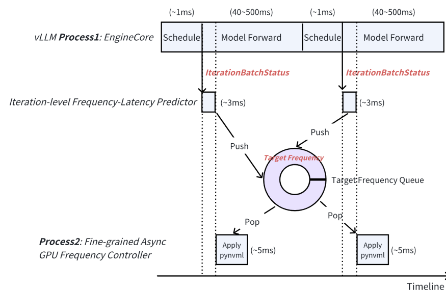
Figure 7. Low-overhead runtime design of EcoInfer. (a) Three-overlap pipelining hides CPU-side scheduling and frequency prediction behind GPU execution, eliminating the GPU stalls present in naive control. (b) A dedicated frequency-controller process applies DVFS decisions asynchronously via pyNVML, decoupling the blocking actuation call from the inference critical path.
