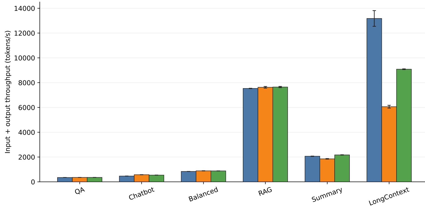
Total Token Throughput
