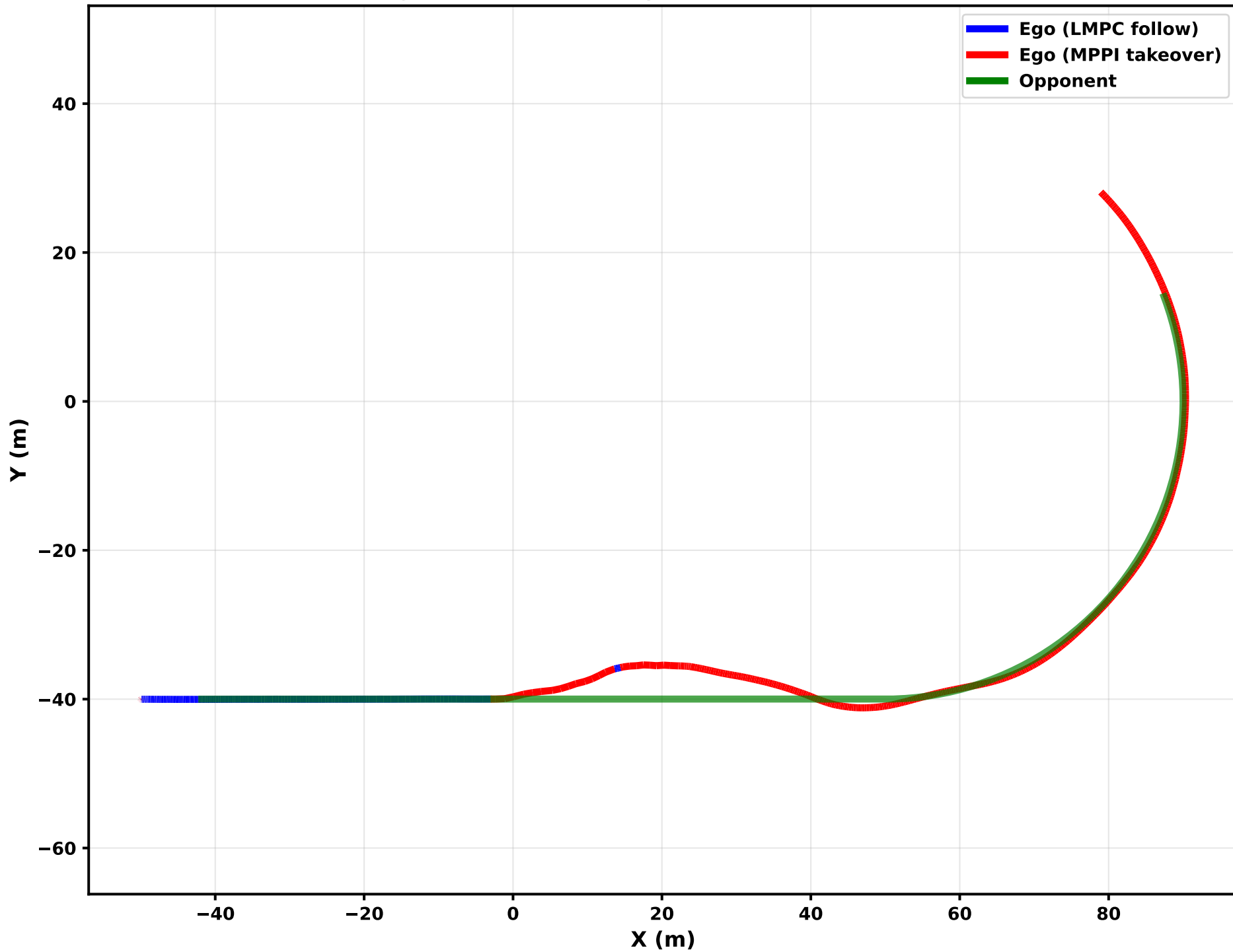
Ego vs Opponent Trajectories (world frame)
