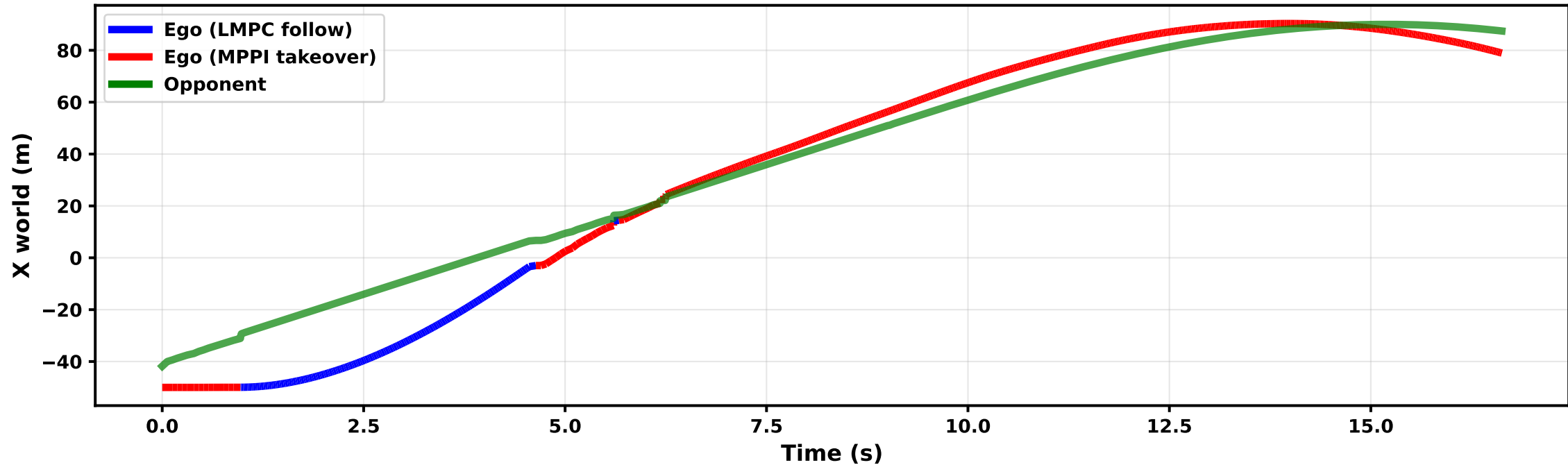
X Position vs Time (world frame)
