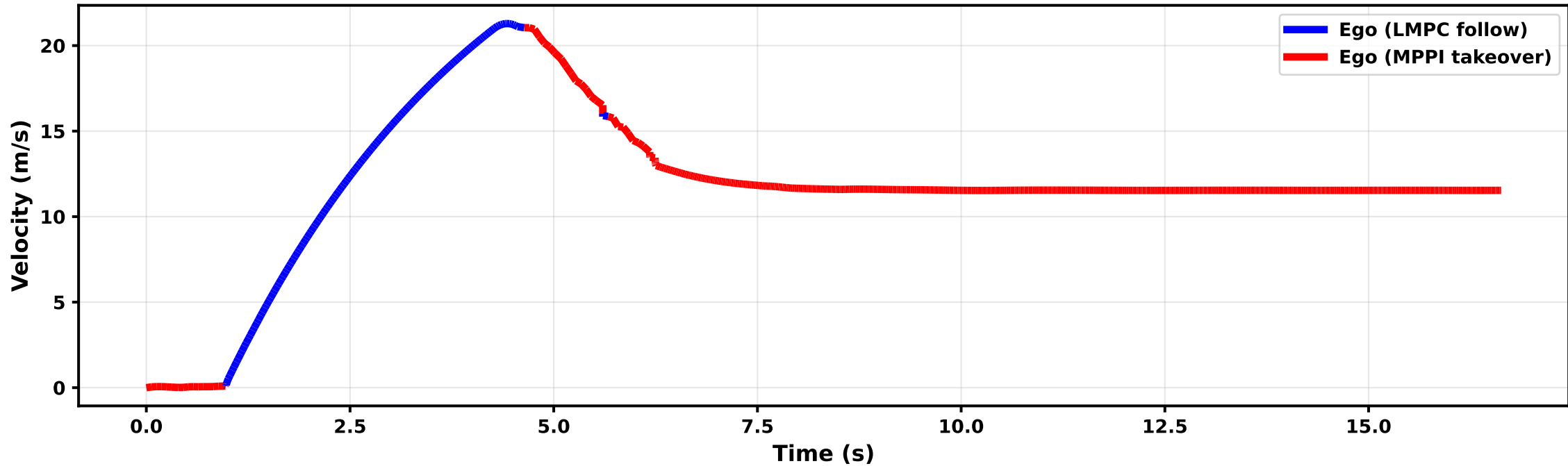
Ego Velocity vs Time
