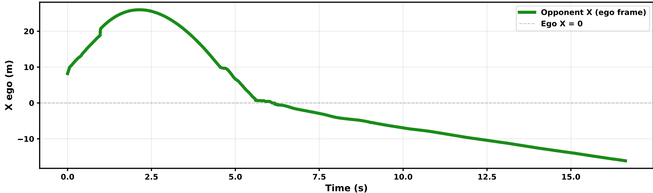
Opponent X in Ego Frame vs Time (+ = ahead)
