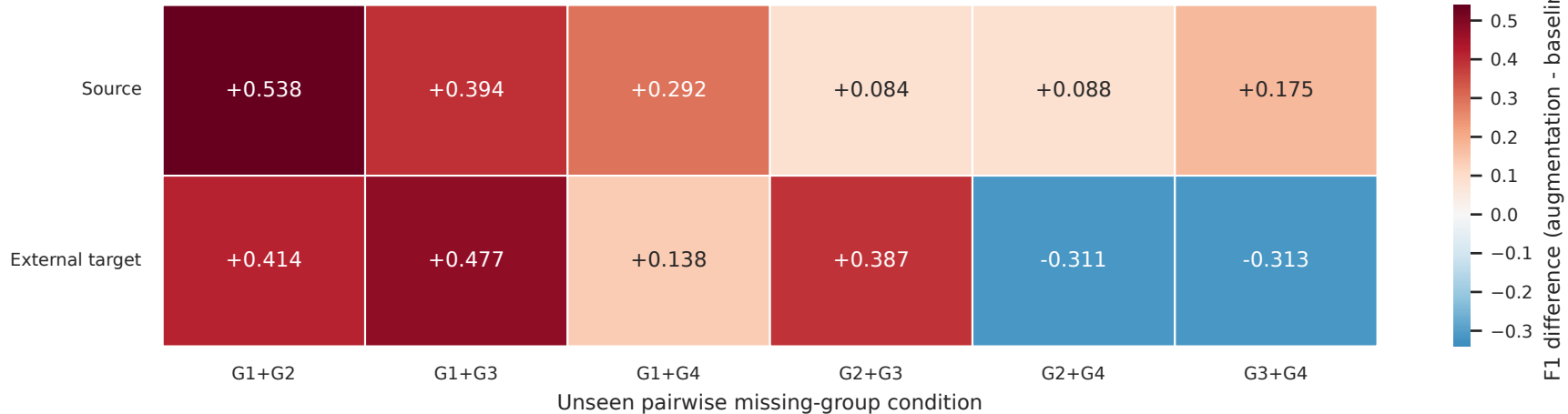
Mask-augmentation benefit is condition dependent under dataset shift
