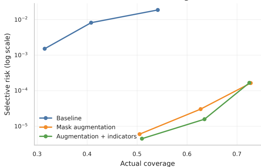
External target risk-coverage
