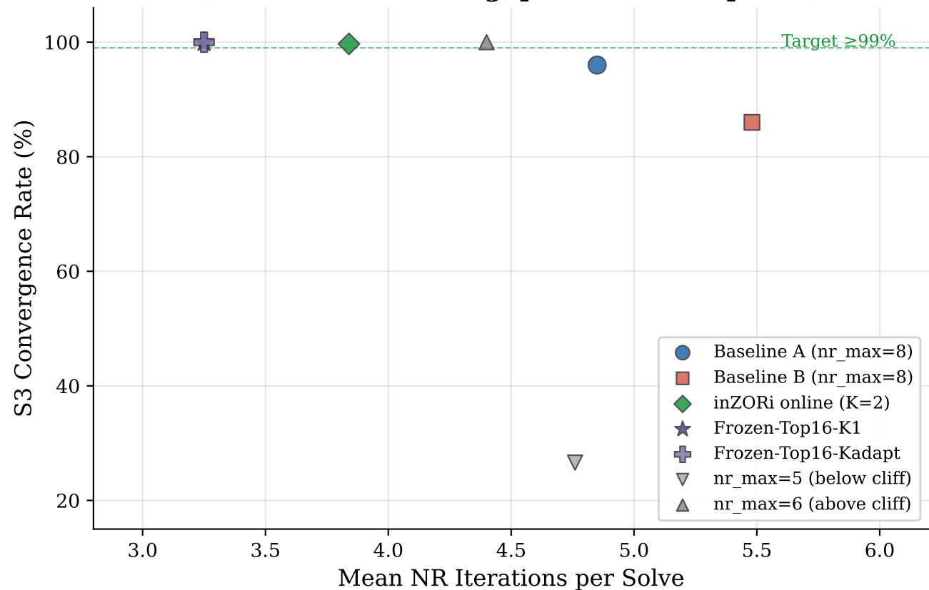
Pareto Frontier: S3 Convergence vs. Iteration Cost (marker size \propto throughput in conv-steps/sec)
