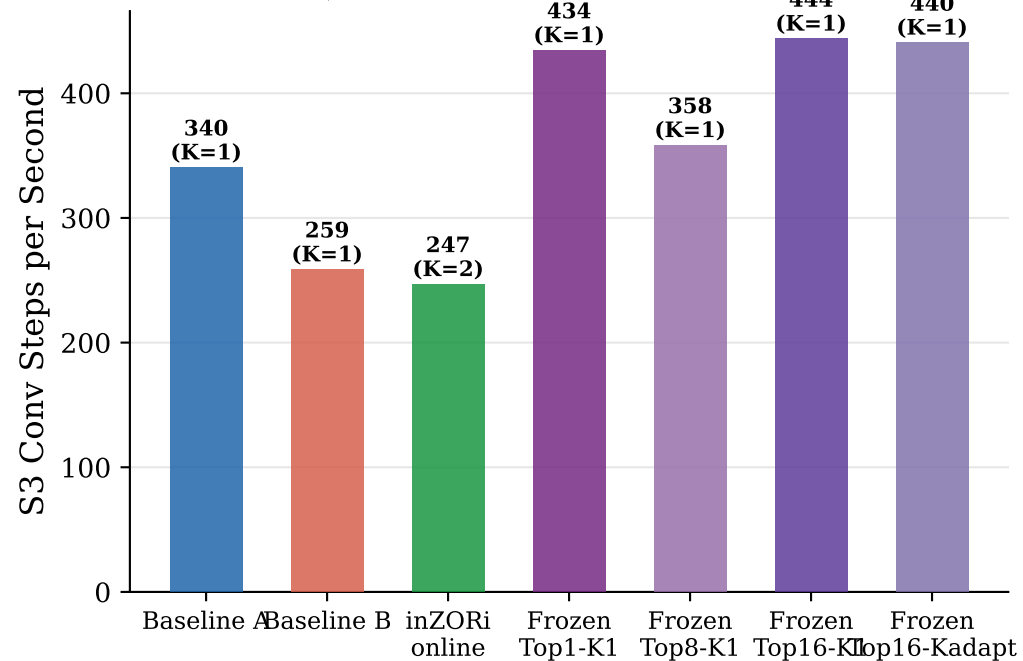
(b) Runtime Throughput (lower K = more efficient)
