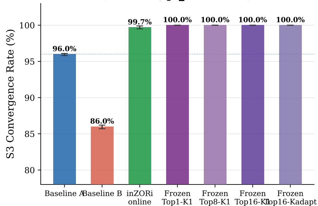
(a) S3 Convergence (20 seeds, pf_interval=1)
