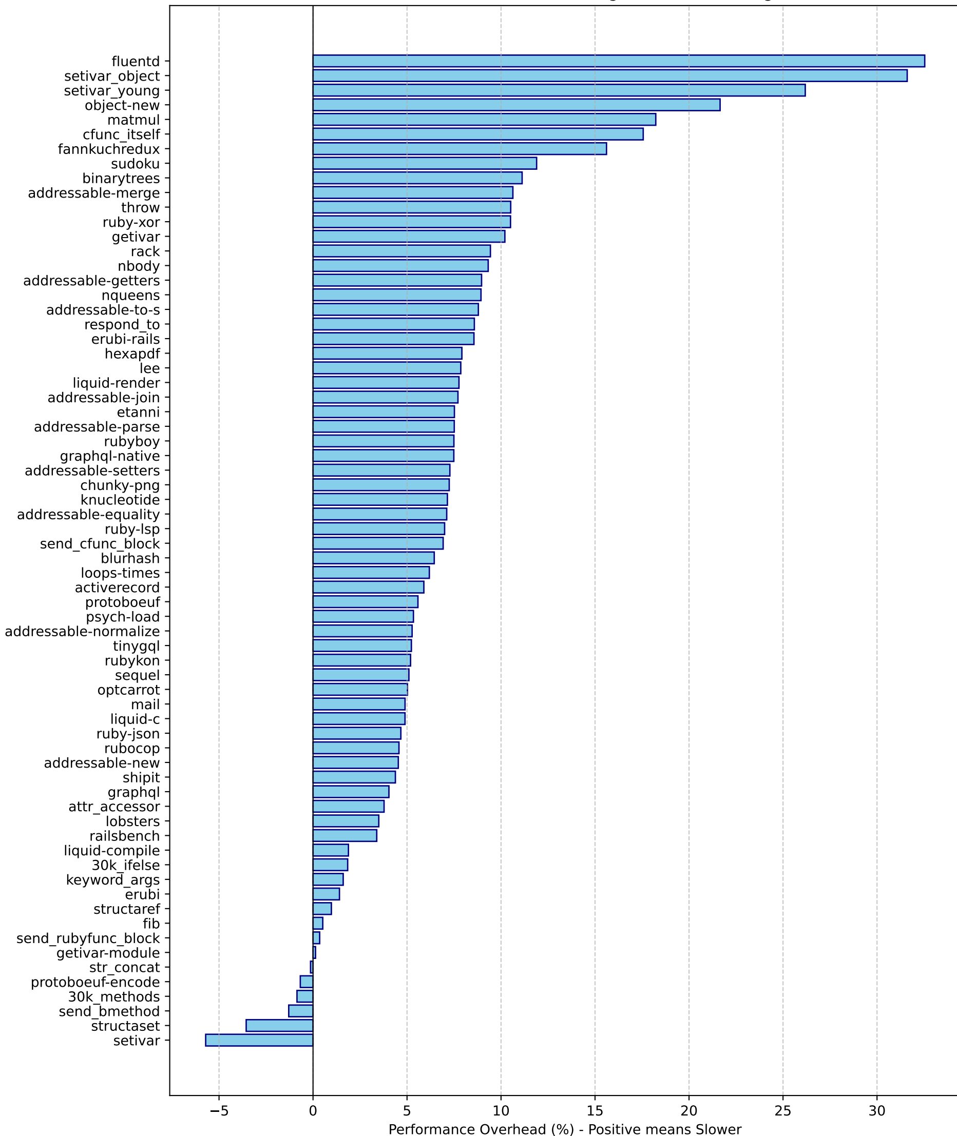
Performance Overhead of Guarding All VALUES vs Original
