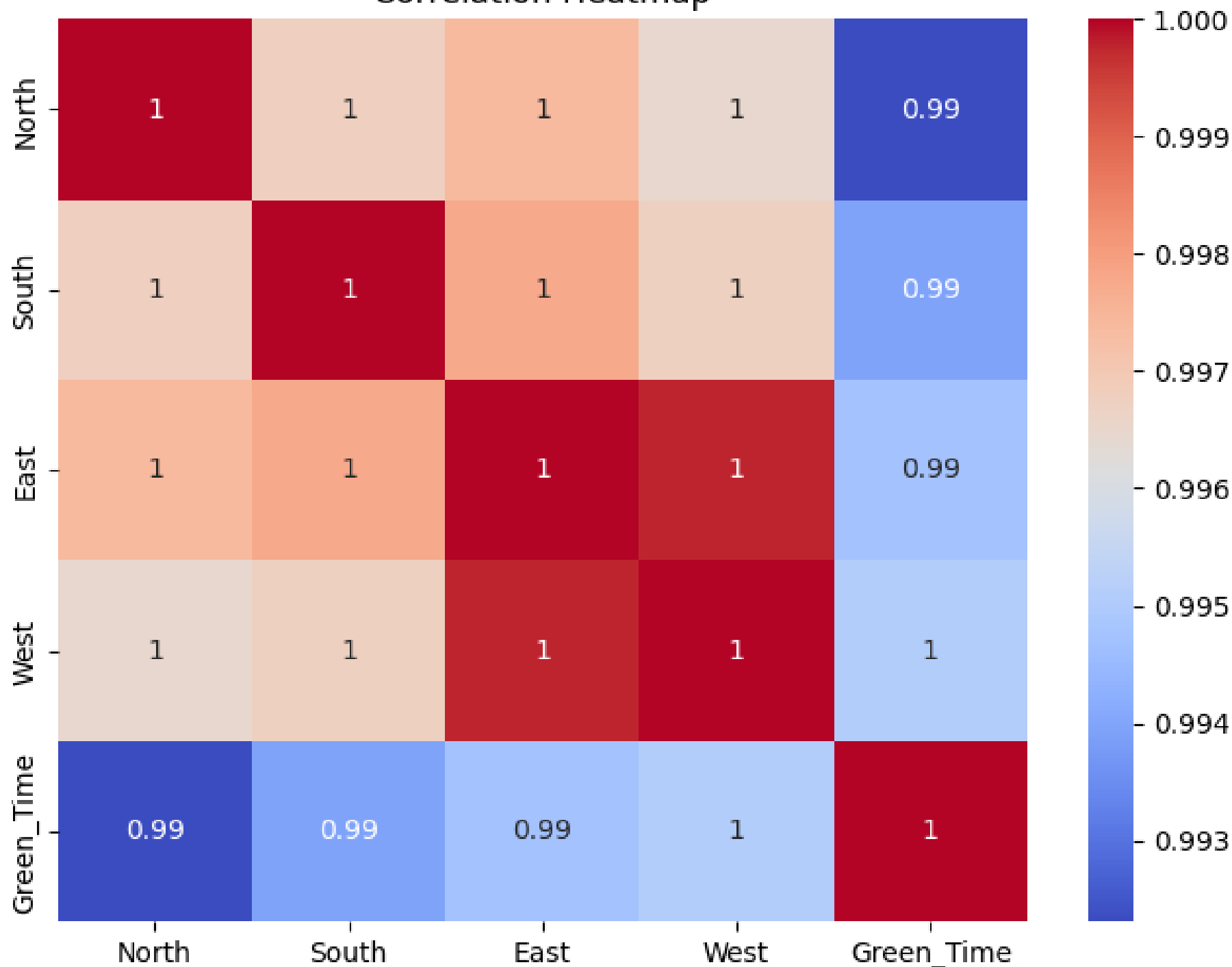
Correlation Heatmap
