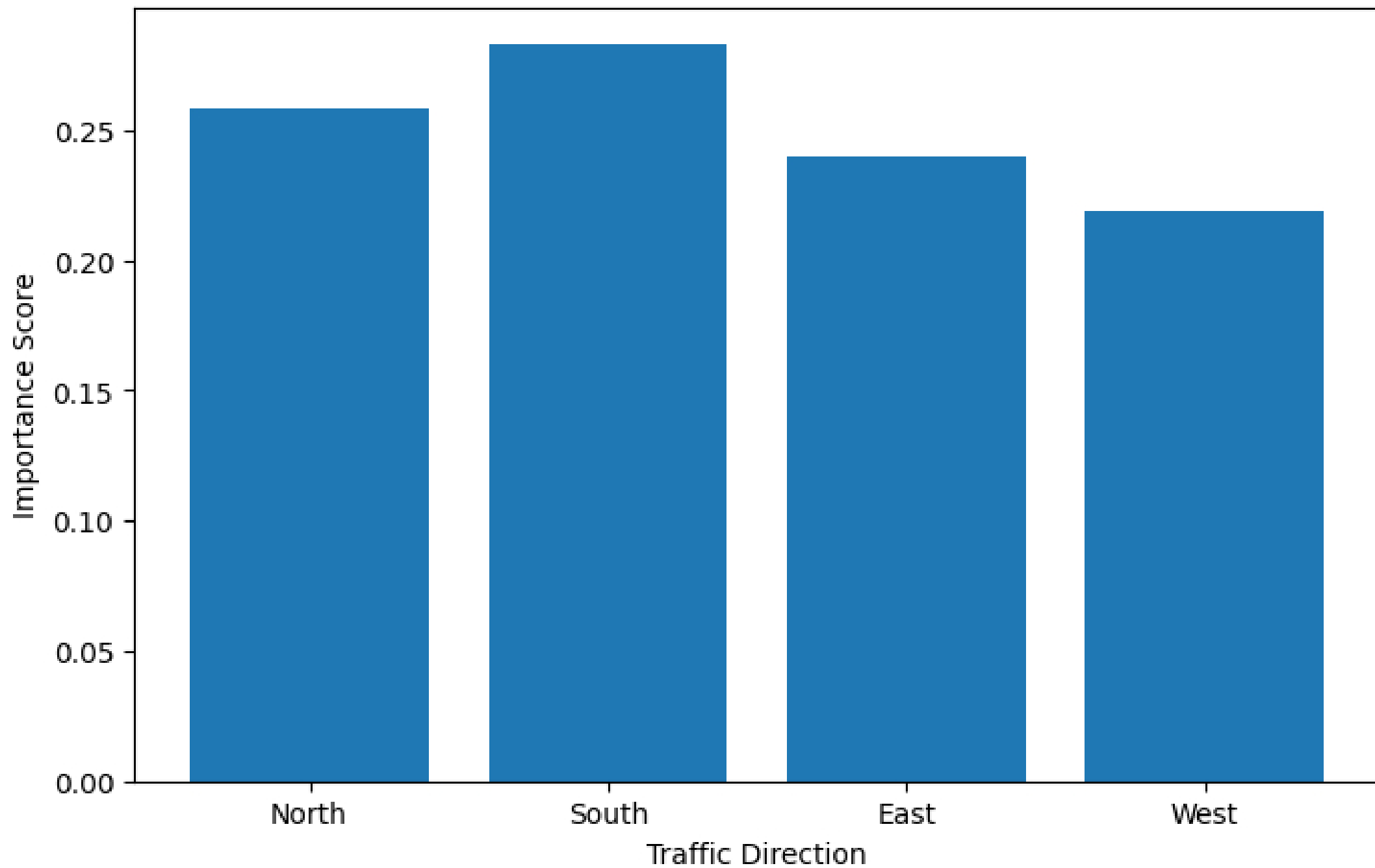
Feature Importance
