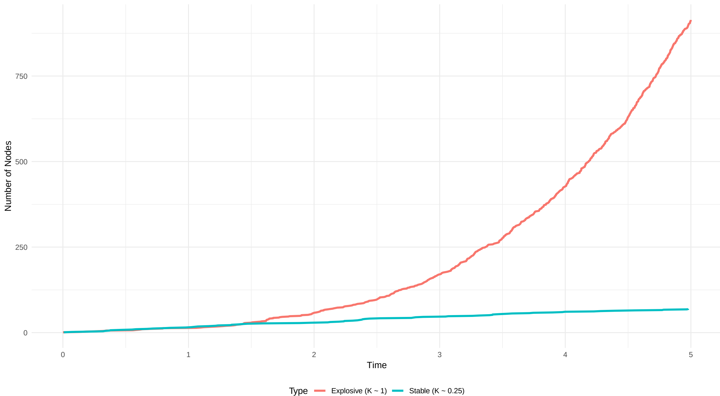
Node Growth Over Time: Explosive vs Stable (BA)
