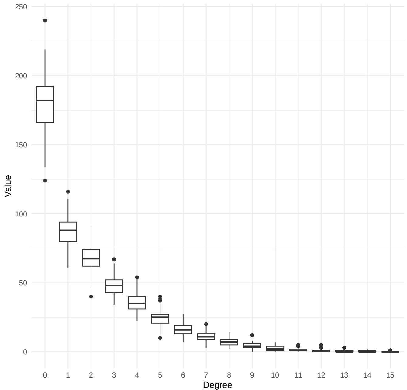
Degree Distribution
