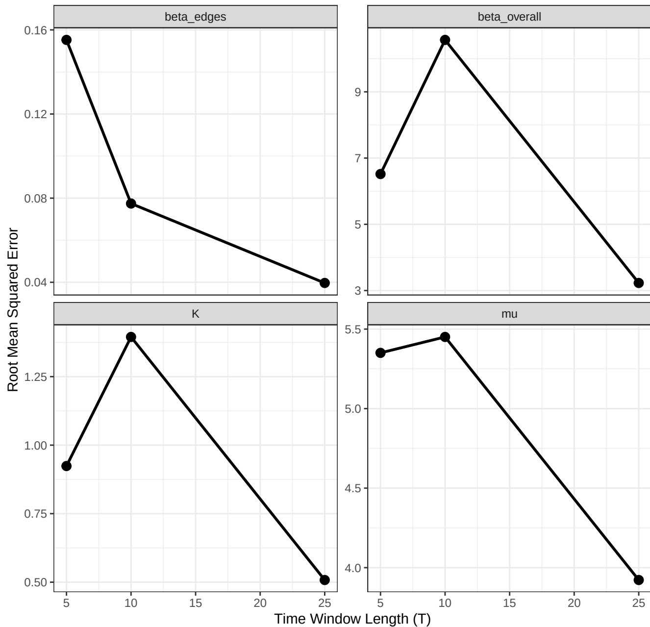
RMSE Decay as Data Increases
