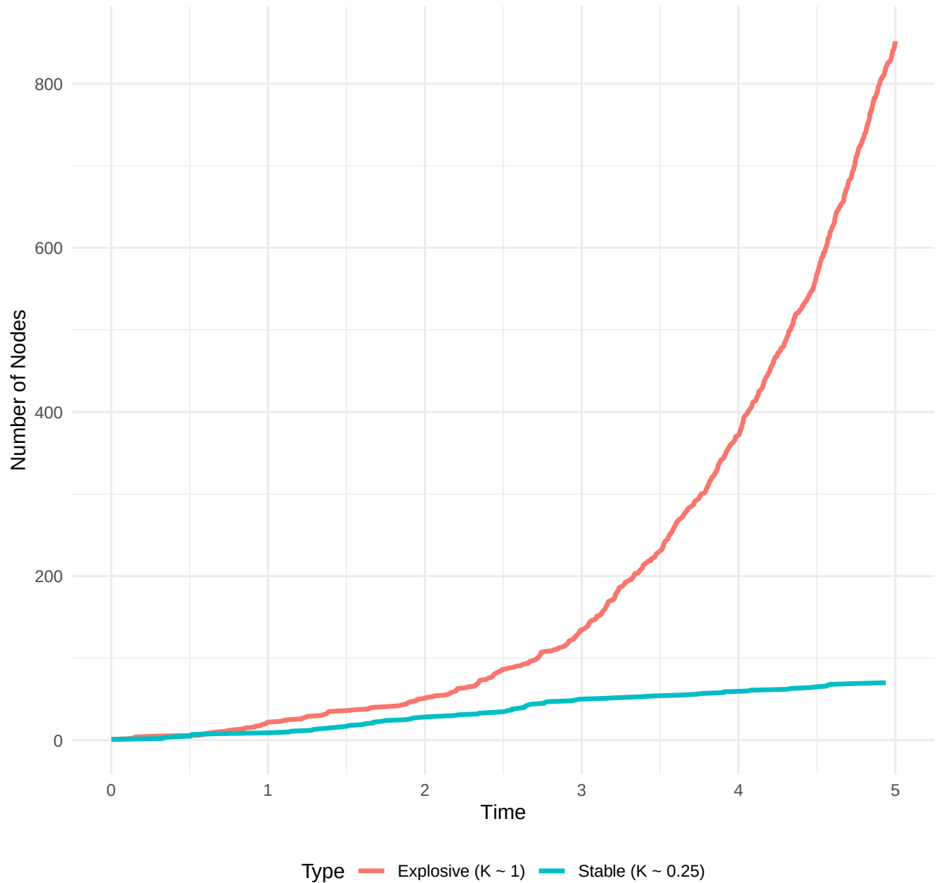
Node Growth Over Time: Explosive vs Stable (BA)
