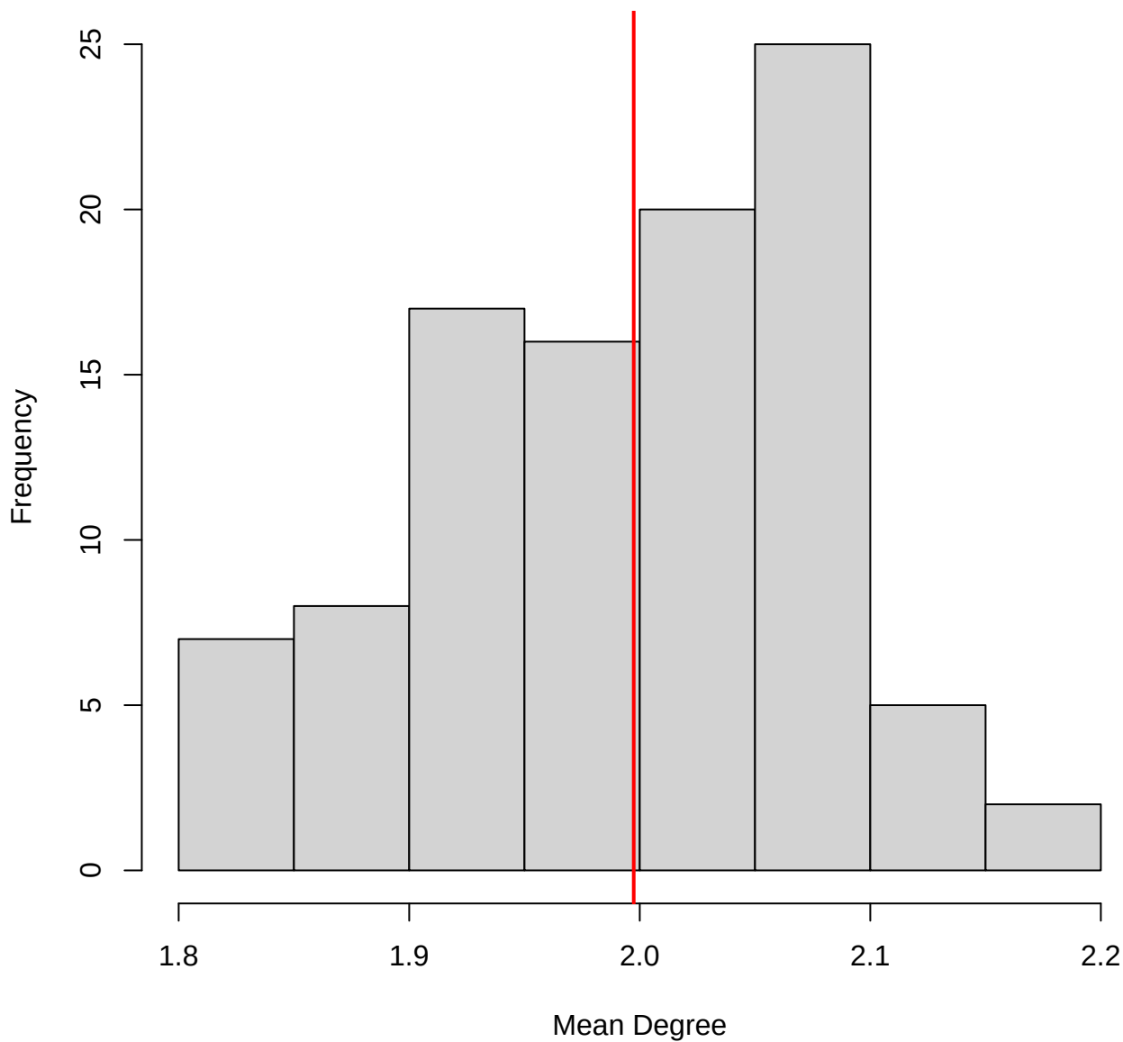
Histogram of Mean Degrees
