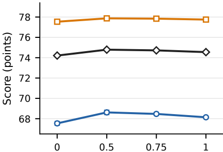
(a) Topology weight \lambda_{\text{topo}}
