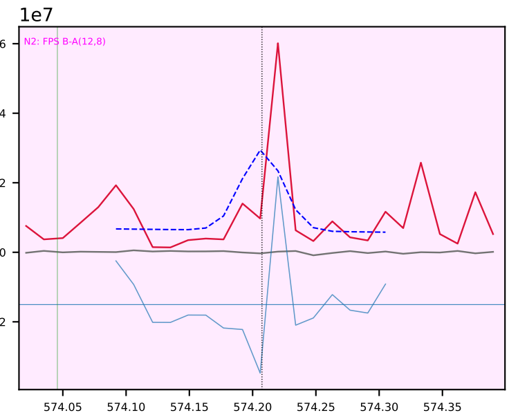
N I 574.20 other19 -> other145 weak, SNR 5, suspect? 1 unexplained feature(s) in fit window; N2 band region: FPS B-A (12,8)
