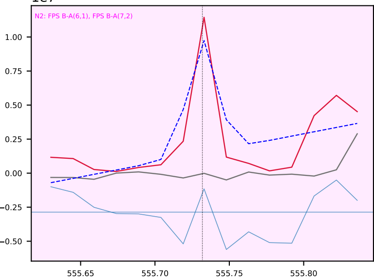
N I 555.74 other14 -> other127 weak, SNR 4, clean? N2 band region: FPS B-A (7,2)/FPS B-A (6,1)
