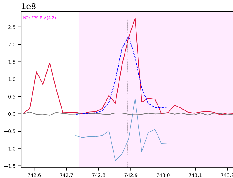
N I 742.88 other22 -> 4d4 weak, SNR 9, suspect? 1 unexplained feature(s) in fit window; N2 band region: FPS B-A (4,2)
