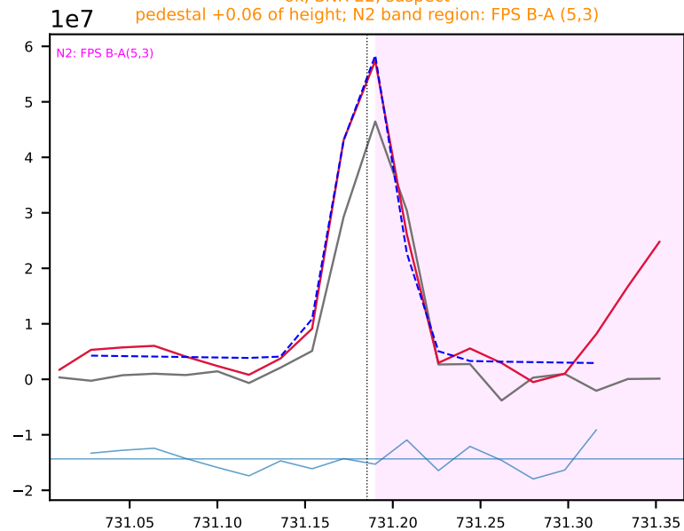
Ar I 731.17 4p4 -> 6s2 ok, SNR 22, suspect pedestal +0.06 of height; N2 band region: FPS B-A (5,3)
