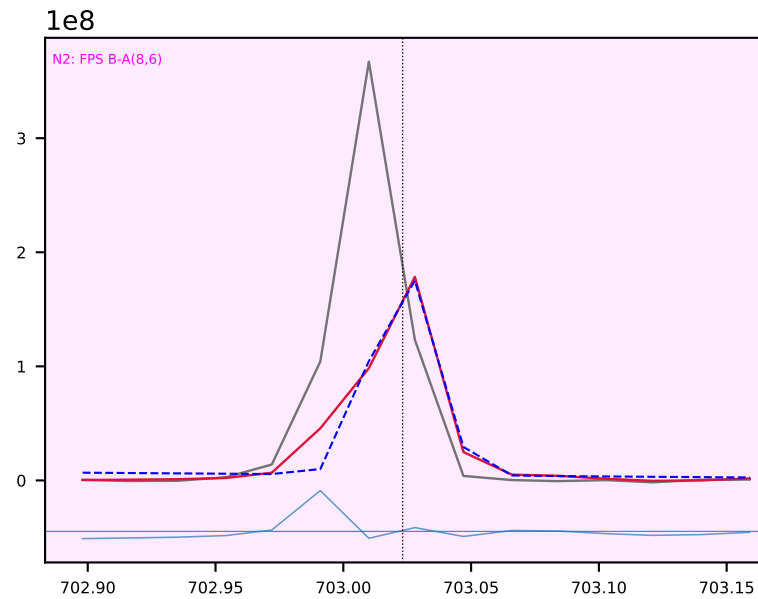
Ar I 703.03 4p2 -> 6s1 ok, SNR 42, suspect reference shift at scan limit; N2 band region: FPS B-A (8,6); mix/pure
