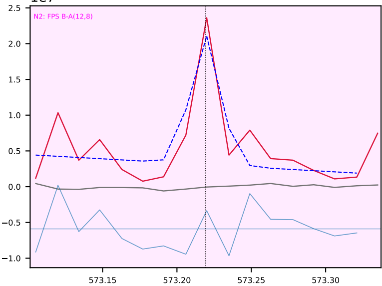
N I 573.21 other21 -> other179 weak, SNR 6, clean? N2 band region: FPS B-A (12,8)
