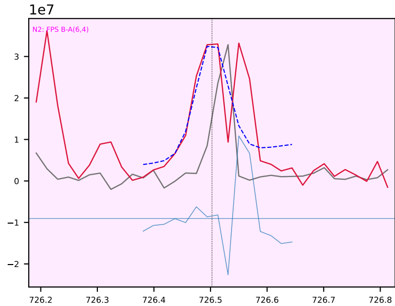
Ar I 726.52 4p4 -> 4d8 weak, SNR 8, contaminated? excess 0.44 (6.0 sigma); hidden line 0.85 x height at 726.557 (N2? FPS
