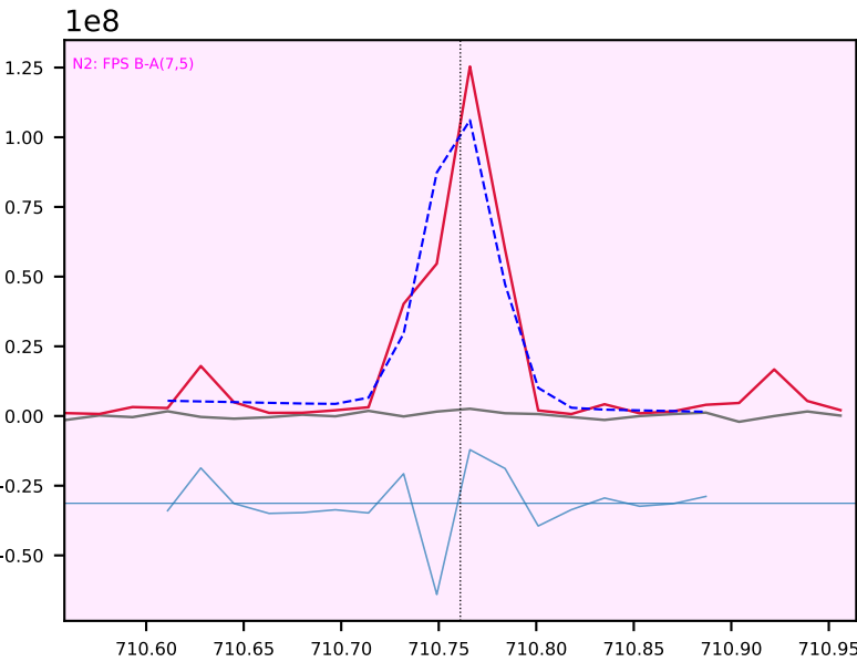
Ar I 710.75 4p3 -> 6s1 ok, SNR 28, suspect N2 band region: FPS B-A (7,5); mix/pure ratio 60.91 vs 30.71 for other
