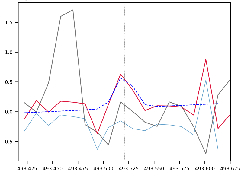
N I 493.51 other9 -> 4p1 weak, SNR 4, clean?
