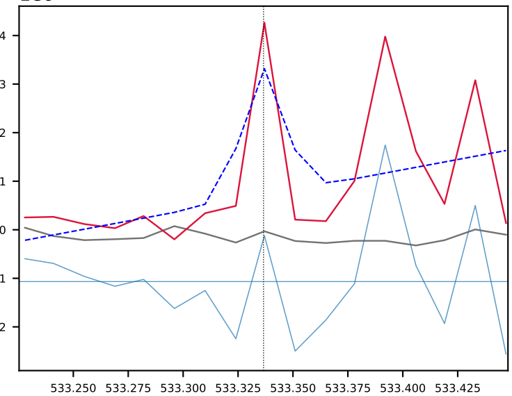
N I 533.34 other21 -> other227 weak, SNR 3, clean?
