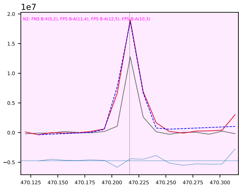
Ar I 470.23 4s4 -> 5p1 ok, SNR 42, contaminated width x1.39 vs pure; excess 0.06 (5.3 sigma); N2 band region: FNS B-X
