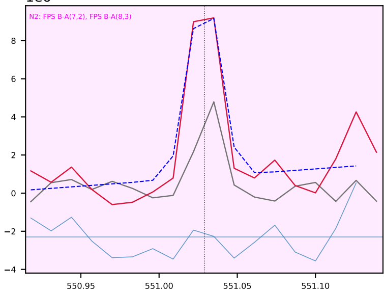
N I 551.02 other21 -> other205 weak, SNR 8, clean? N2 band region: FPS B-A (8,3)/FPS B-A (7,2)
