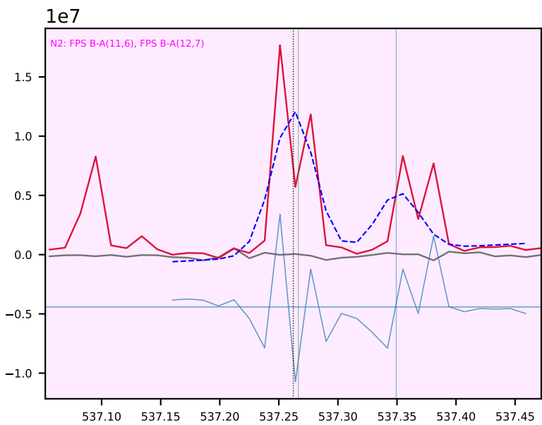
N I 537.26 other12 -> 4p3 ok, SNR 10, suspect 2 unexplained feature(s) in fit window; N2 band region: FPS B-A (12,7)
