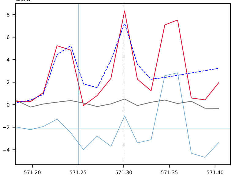
N I 571.31 other21 -> other181 weak, SNR 3, clean?
