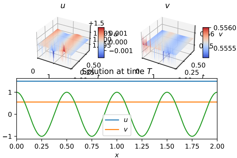
(a) Numerical solution of the Schnackenberg model.
