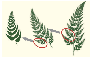
Figure 1: Fractal pattern in fern leaf
