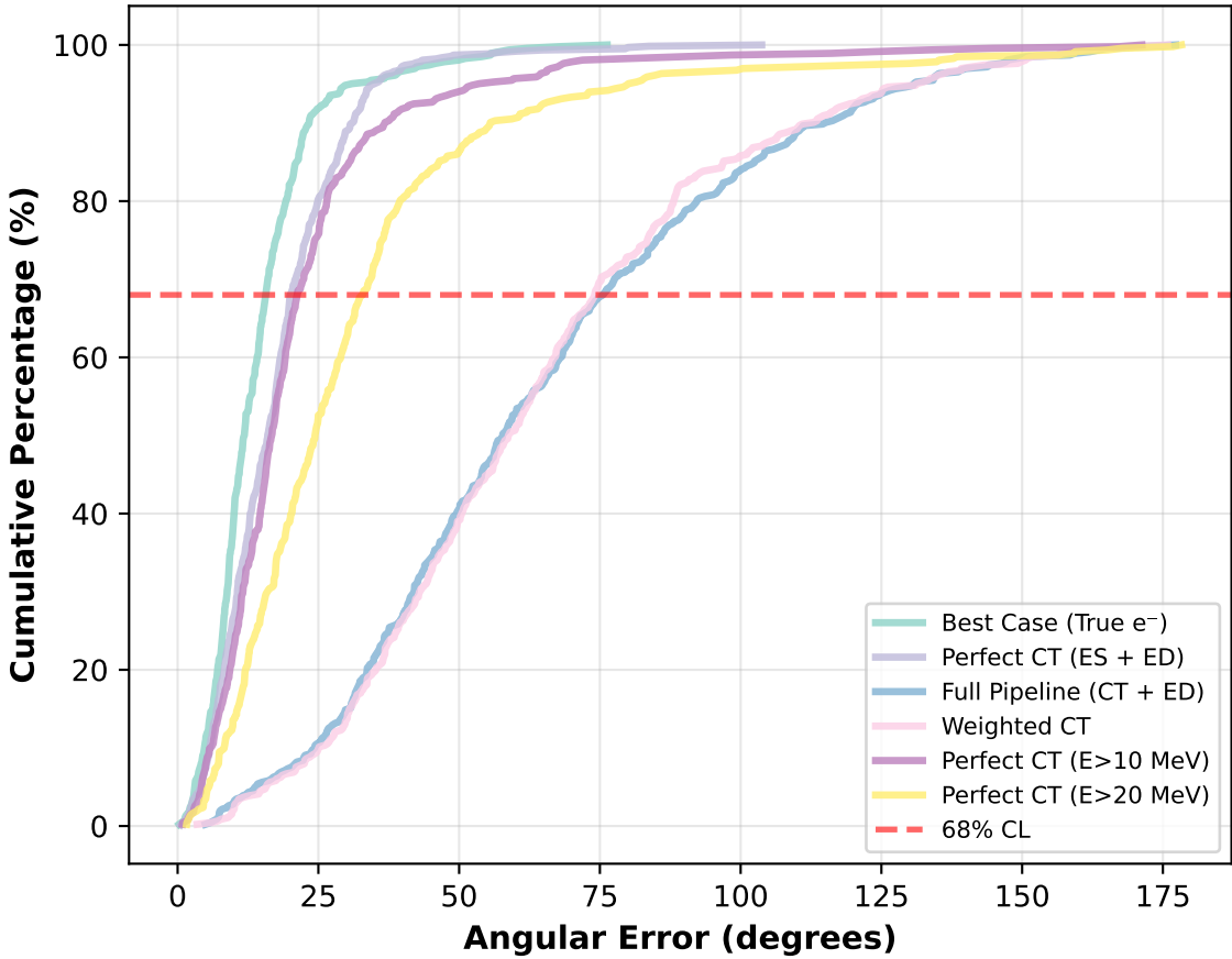
Cumulative Distribution
