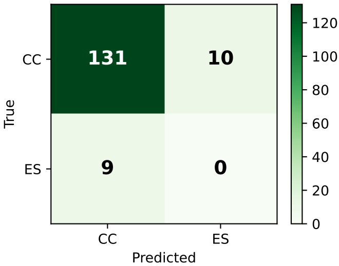
Confusion Matrix
