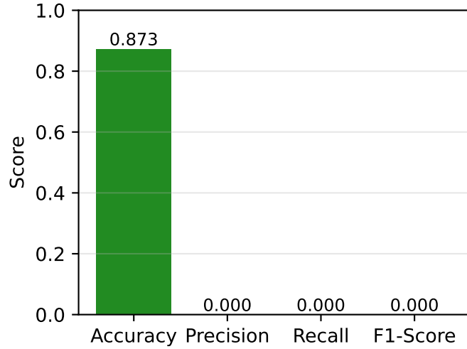
Performance Metrics
