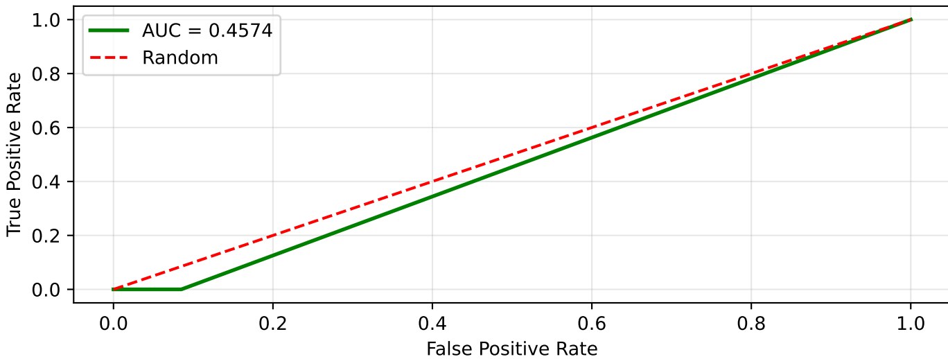
ROC Curve
