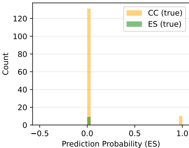
Prediction Distribution
