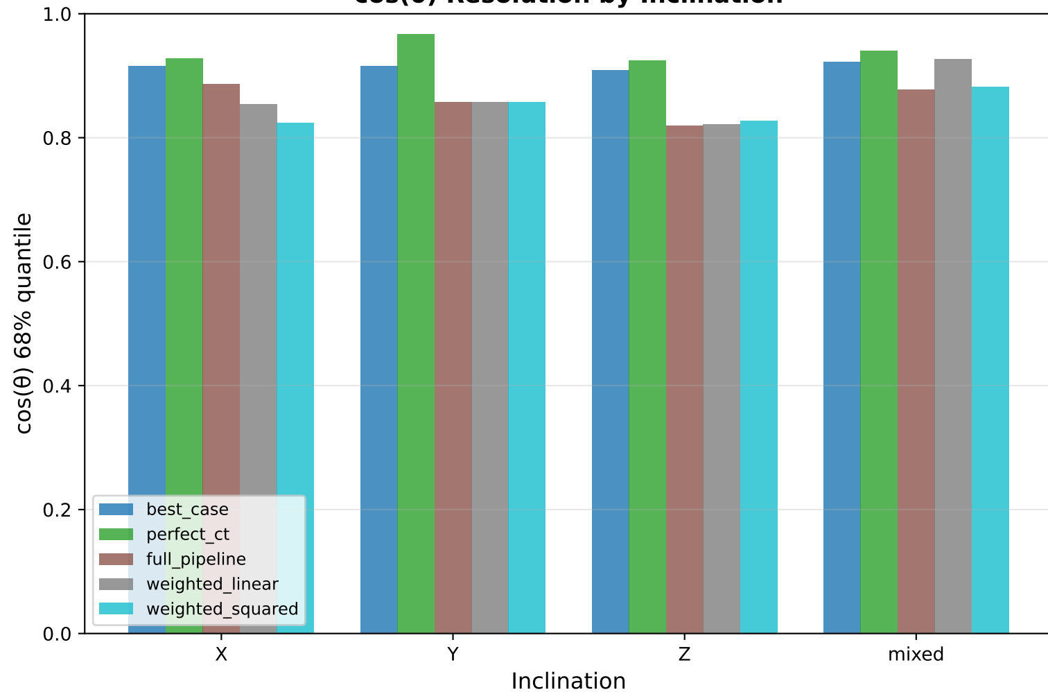
cos( \theta ) Resolution by Inclination
