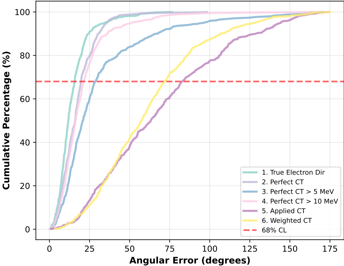
Cumulative Distribution
