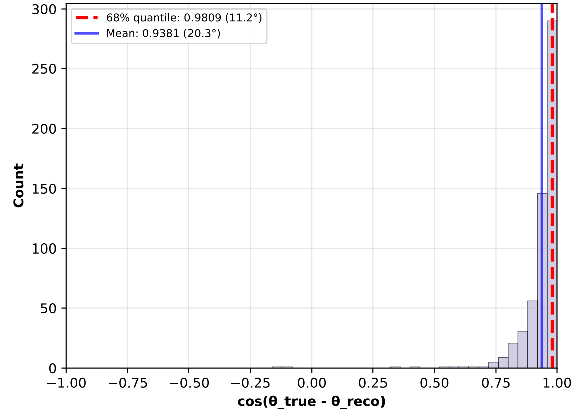
5. Applied CT ( N_{\text{cats}}=567 , N_{\text{ES}}\approx 0 )
