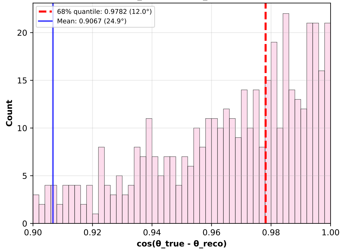
4. Perfect CT > 10 MeV ( N_{\text{cats}}=567 , N_{\text{ES}}\approx 0 )
