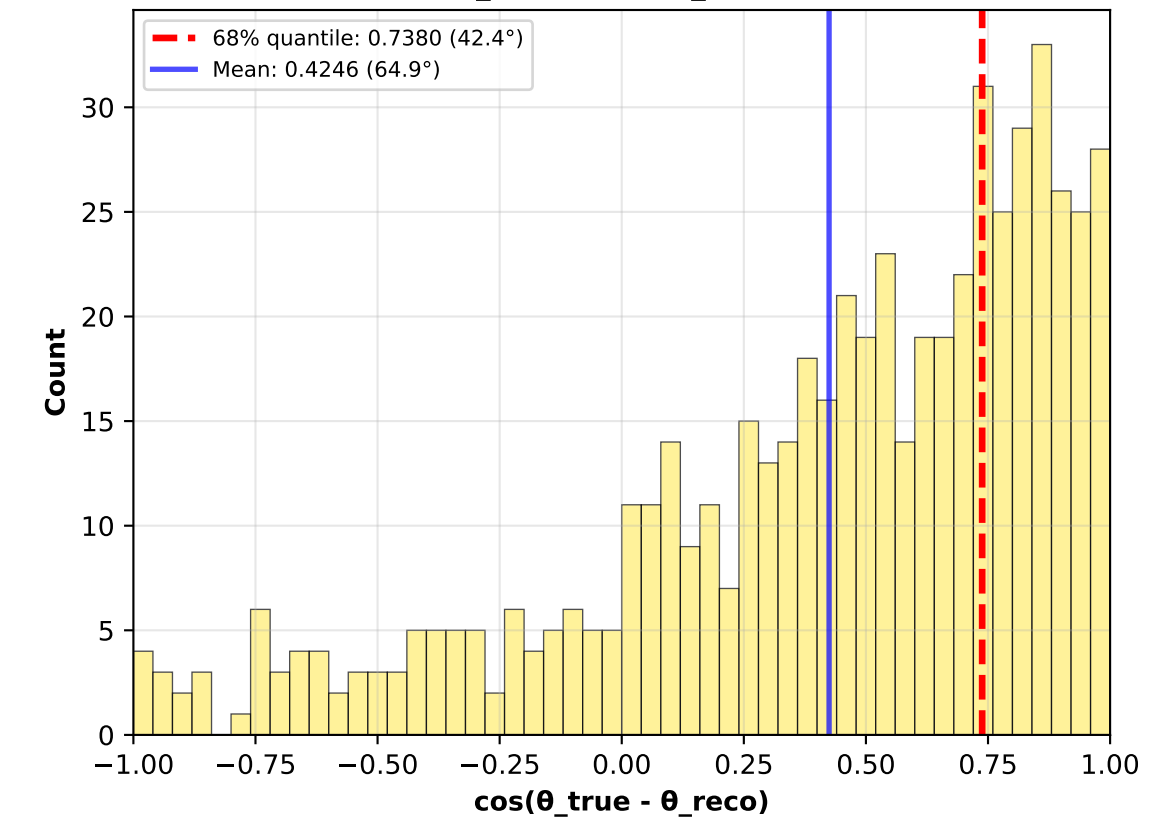
6. Weighted CT ( N_{\text{cats}}=567 , N_{\text{ES}}\approx 0 )
