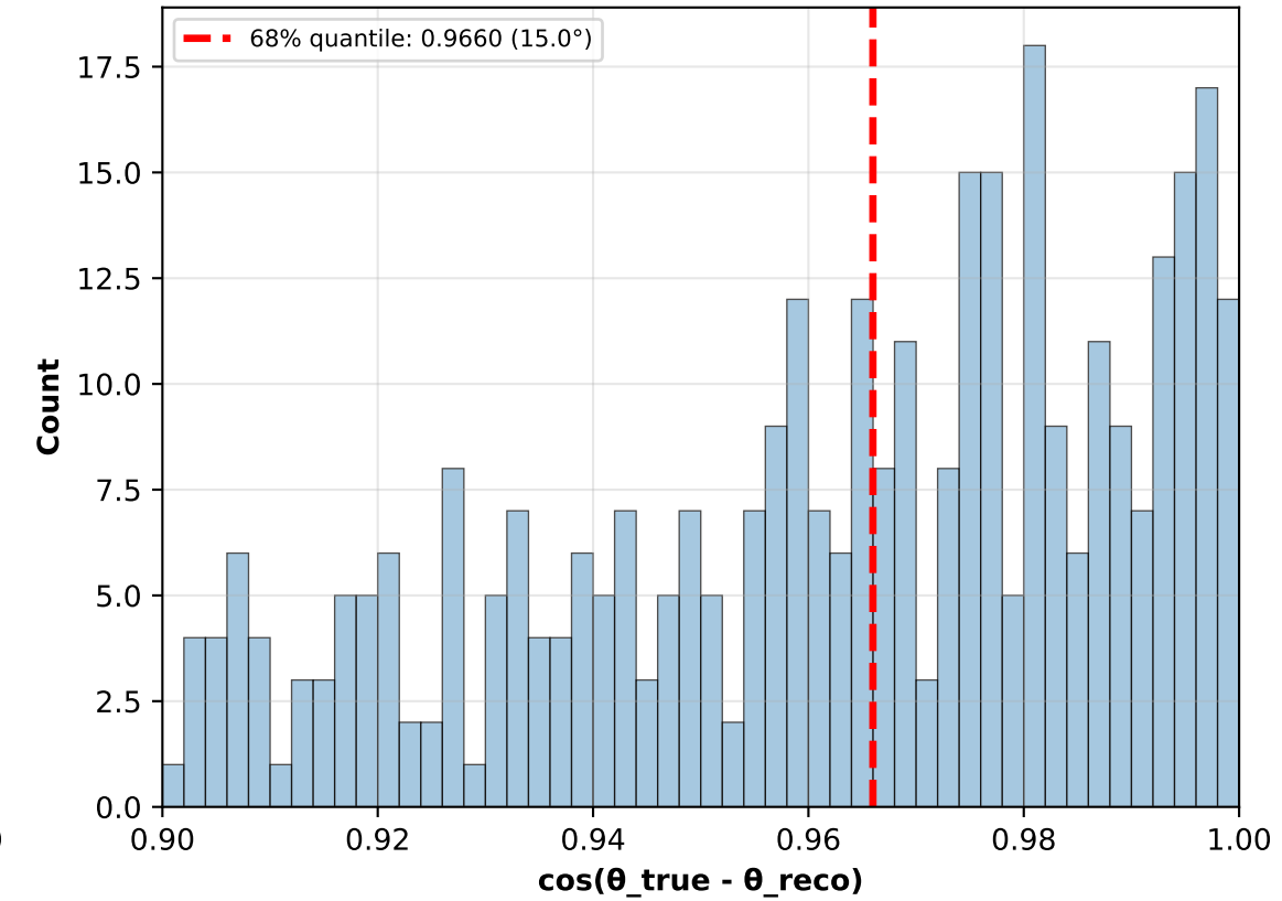
6. Weighted CT ( N_{\text{cats}}=567 , N_{\text{ES}}\approx 0 )
