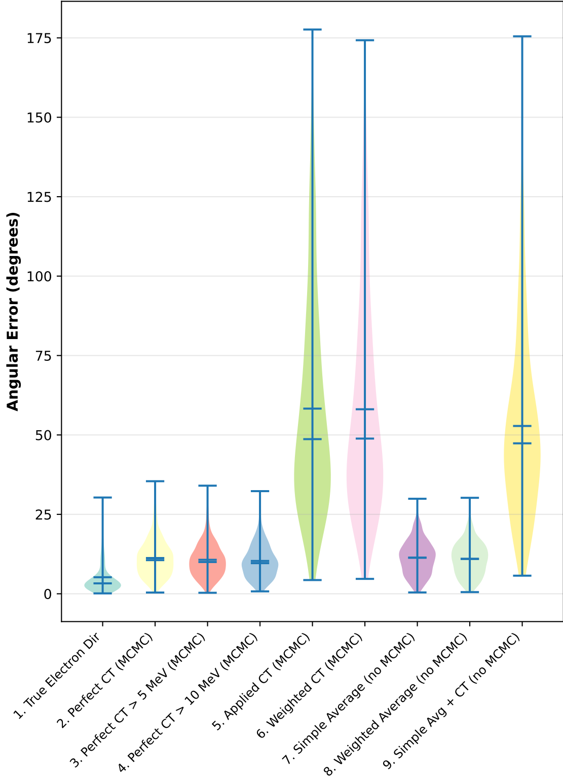
Distribution Shapes
