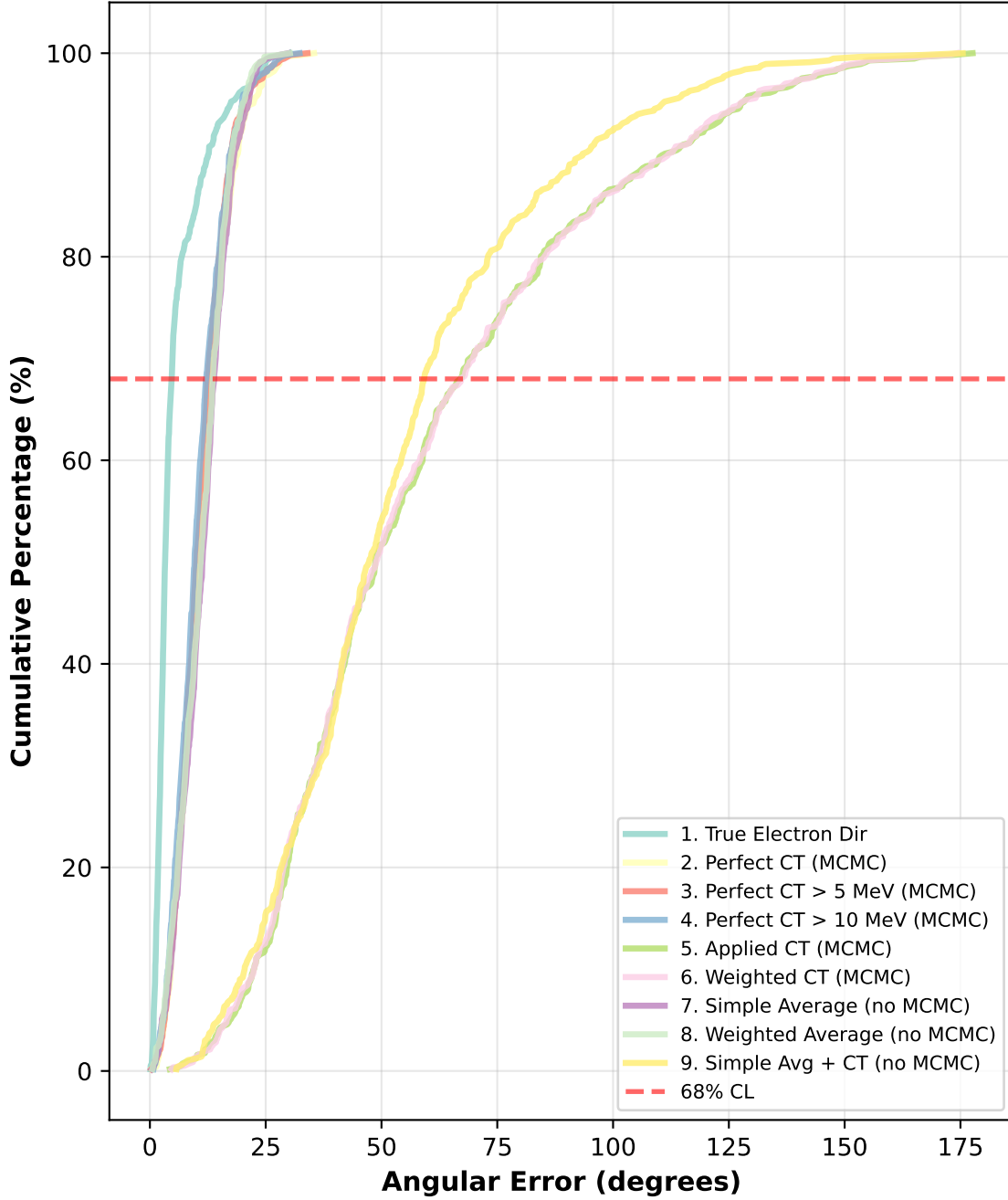
Cumulative Distribution
