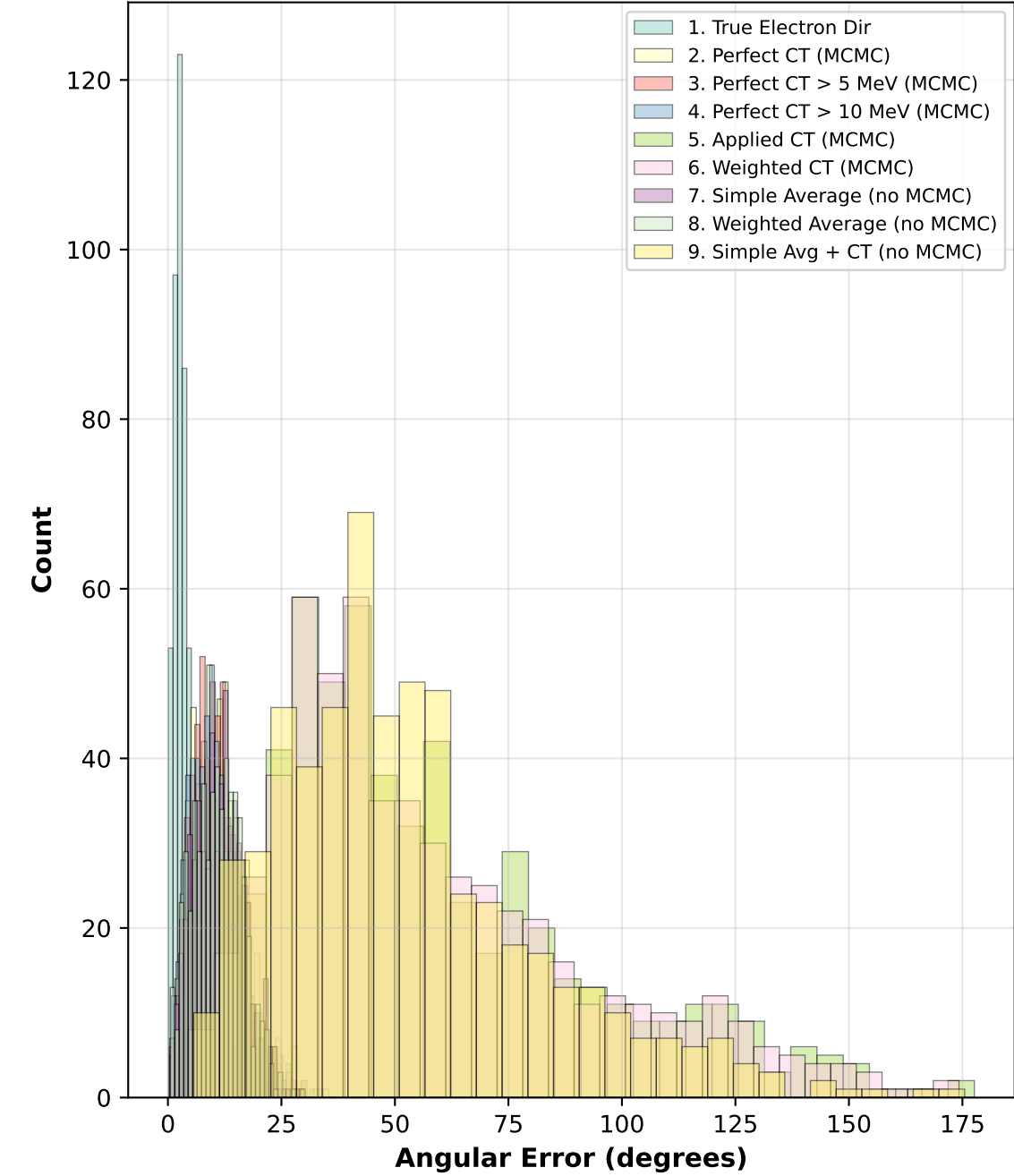
Distribution Overlay
