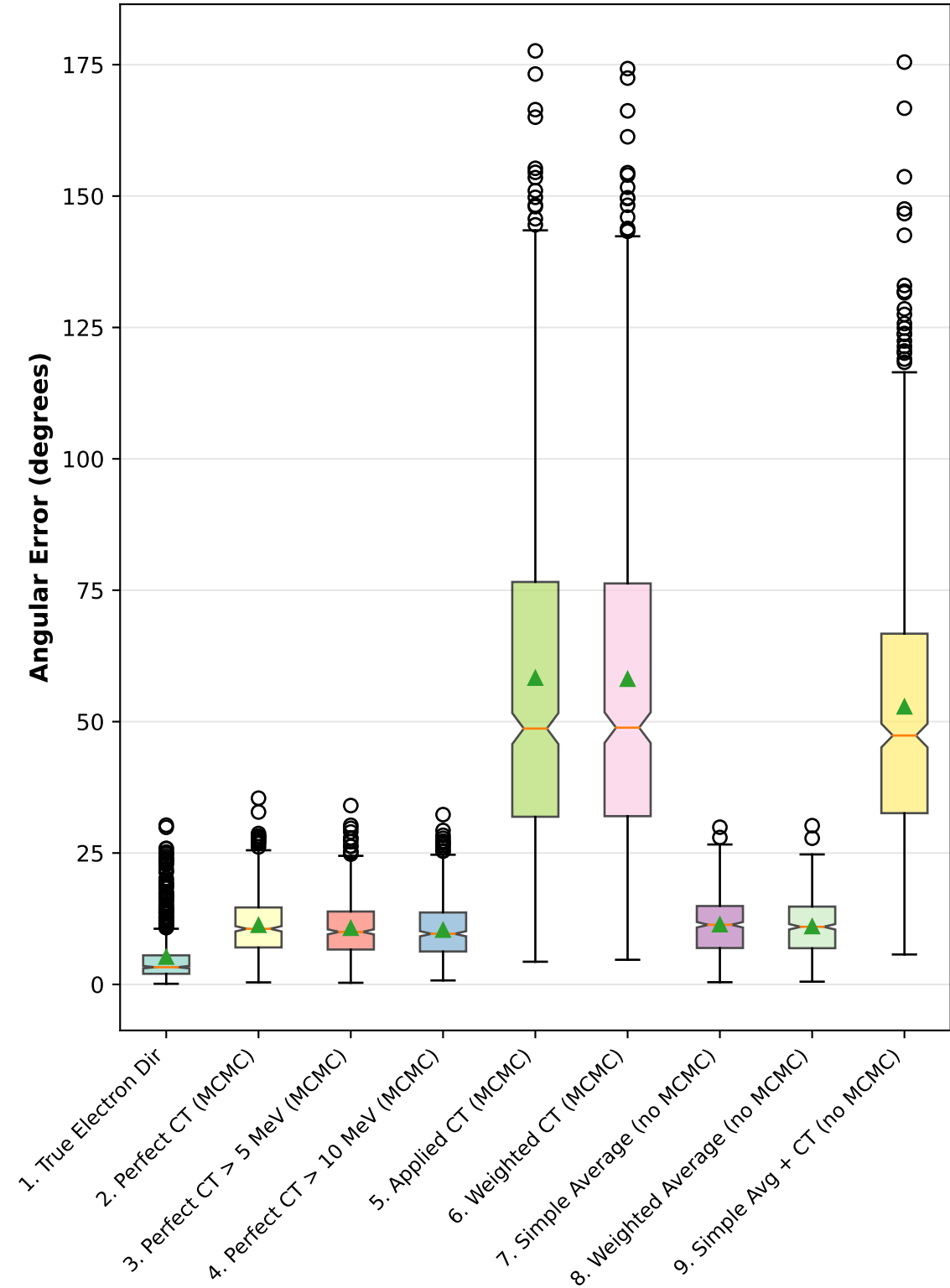
Distribution Overlay
