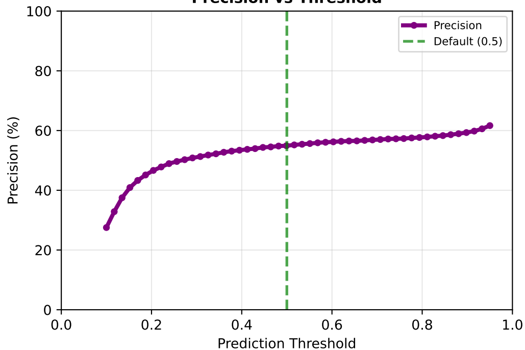
Precision vs Threshold
