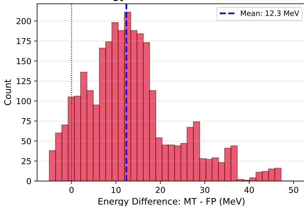
FP vs MT Energy (Split Track Test)
