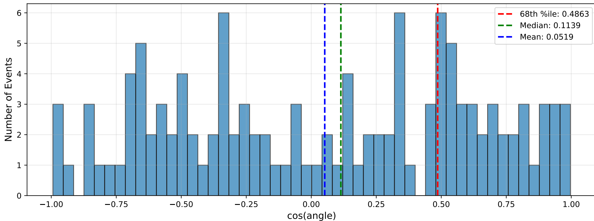
Distribution of \cos(\text{angle}) Between True and Reconstructed
