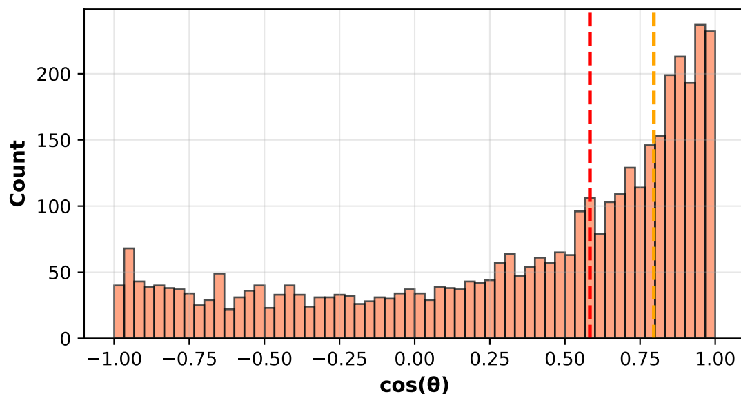
Cosine Distribution
