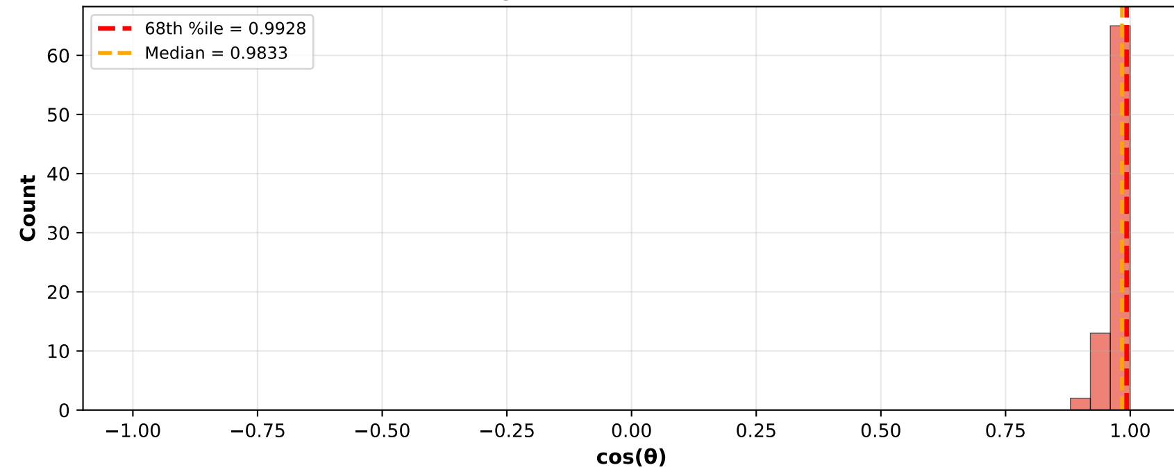
Y-aligned: Cosine Distribution
