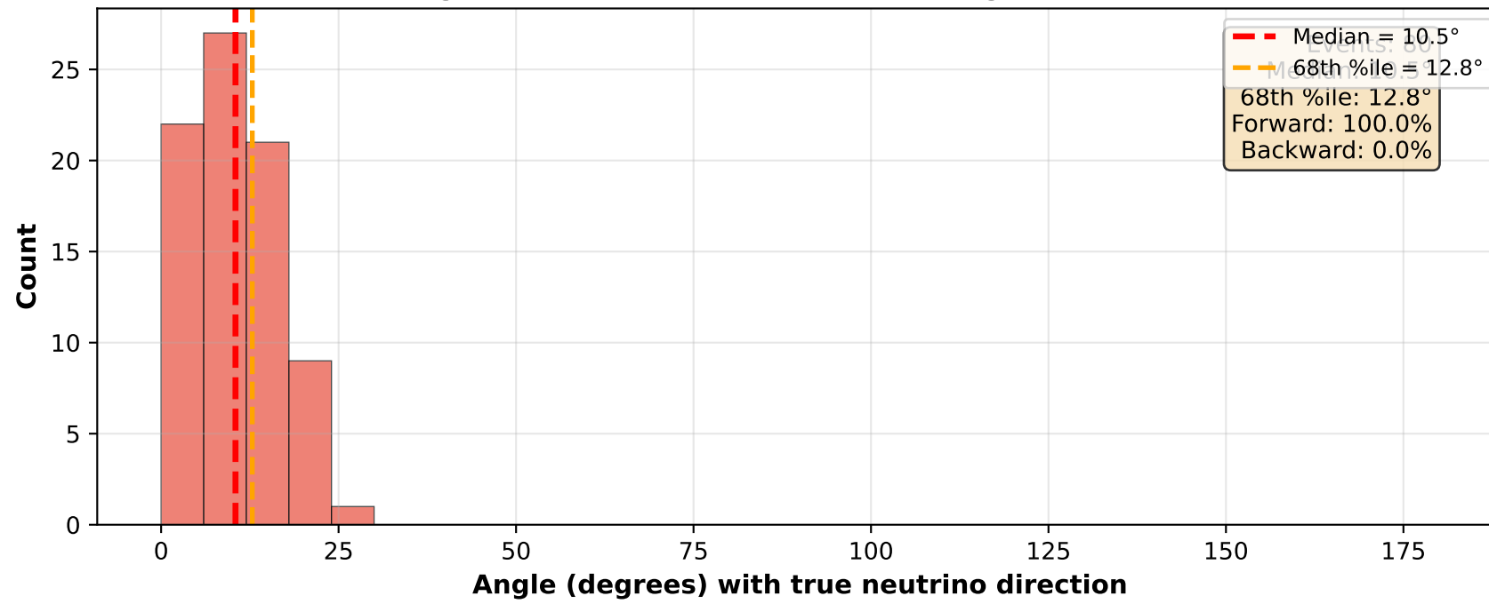
Y-aligned (within \pm 30.0^\circ of Y-axis): Angle Distribution
