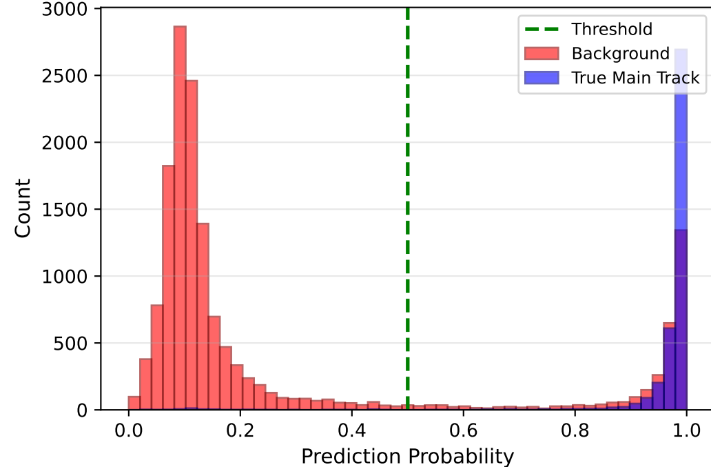
Distribution of MT Predictions
