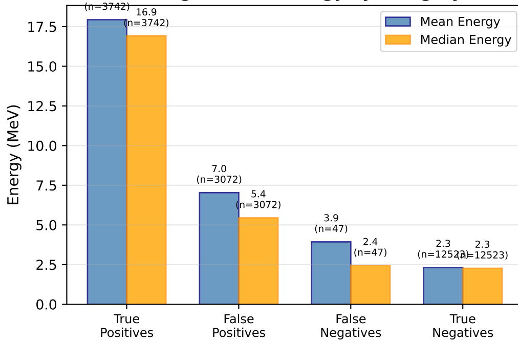
Average Cluster Energy by Category
