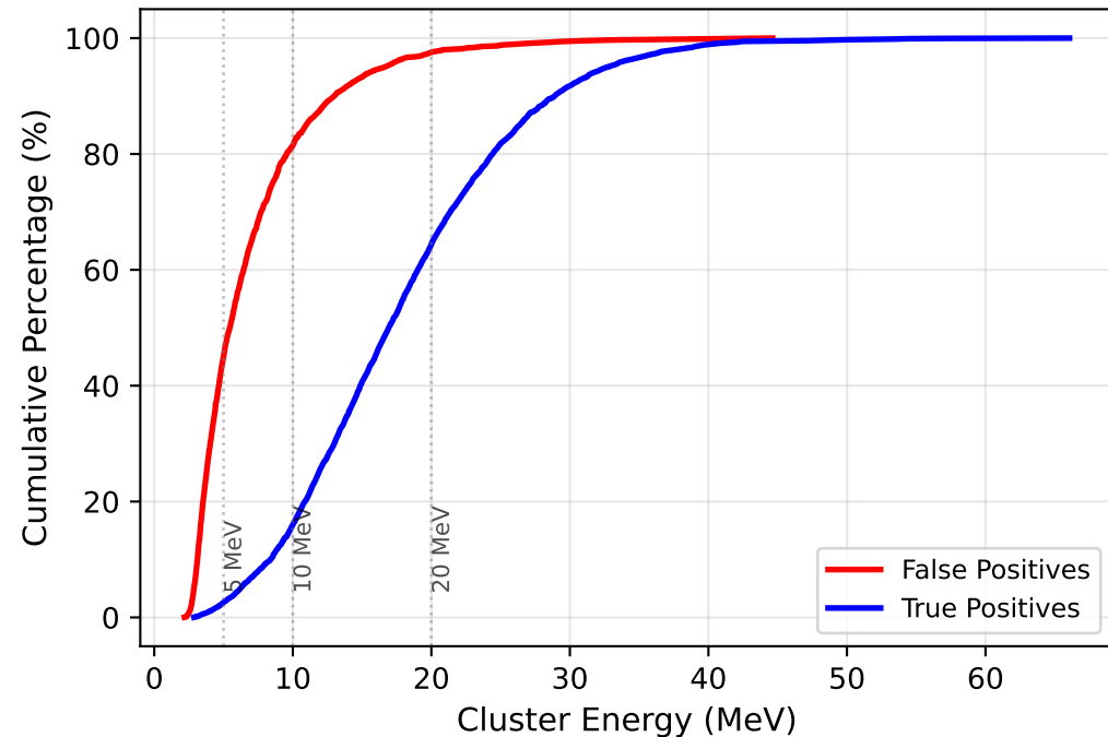
Distribution of MT Predictions
