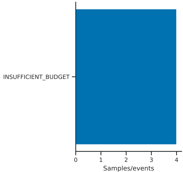
Inconclusive
