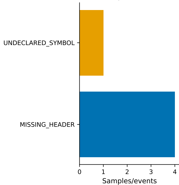
Compile Failure
