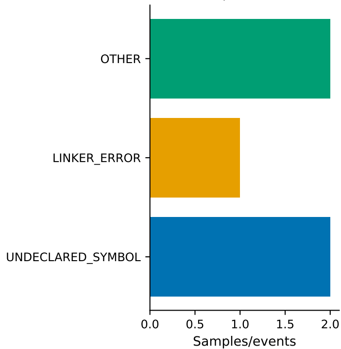
Compile Failure
