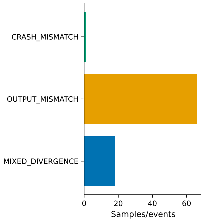
Behavioral Divergence
