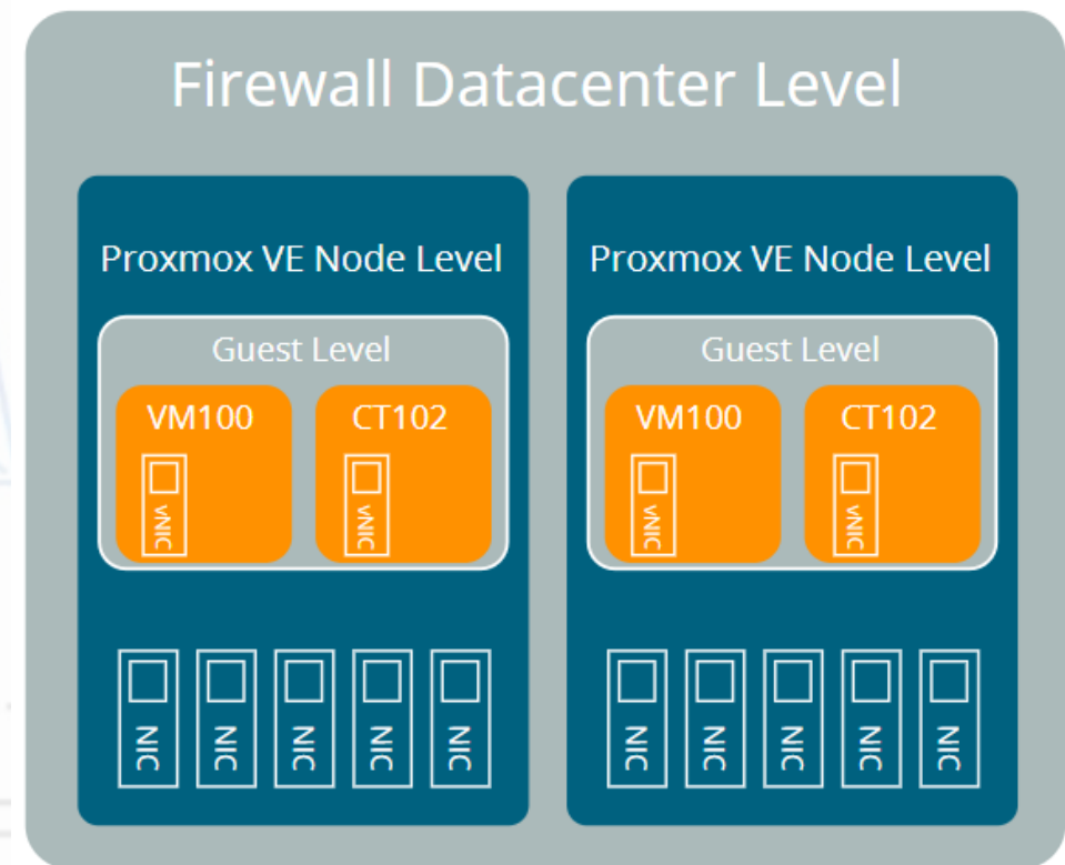
Proxmox Firewall
