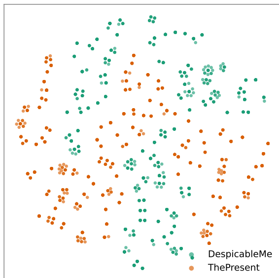
V-JEPA-2: Movie
