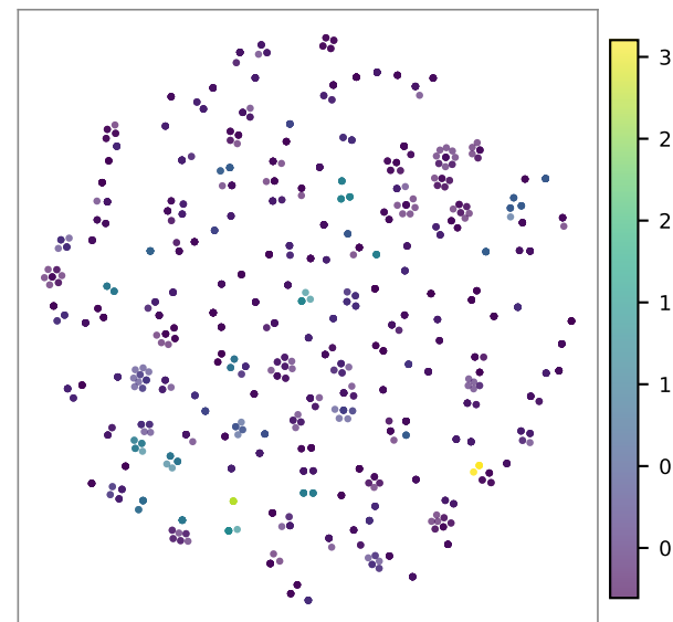
V-JEPA-2: narrative_event_score
