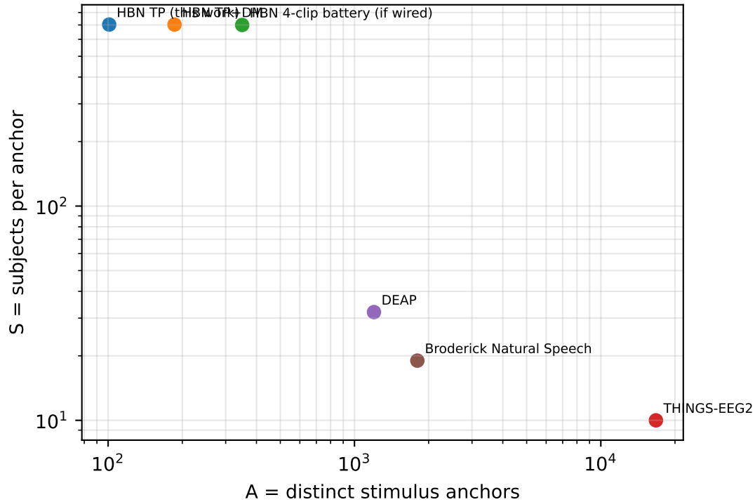
Naturalistic EEG design space (the empty corner)
