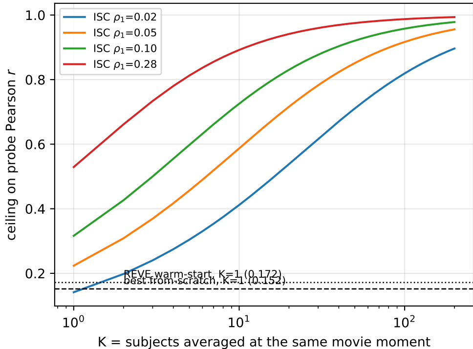
Cross-subject averaging raises the ceiling
