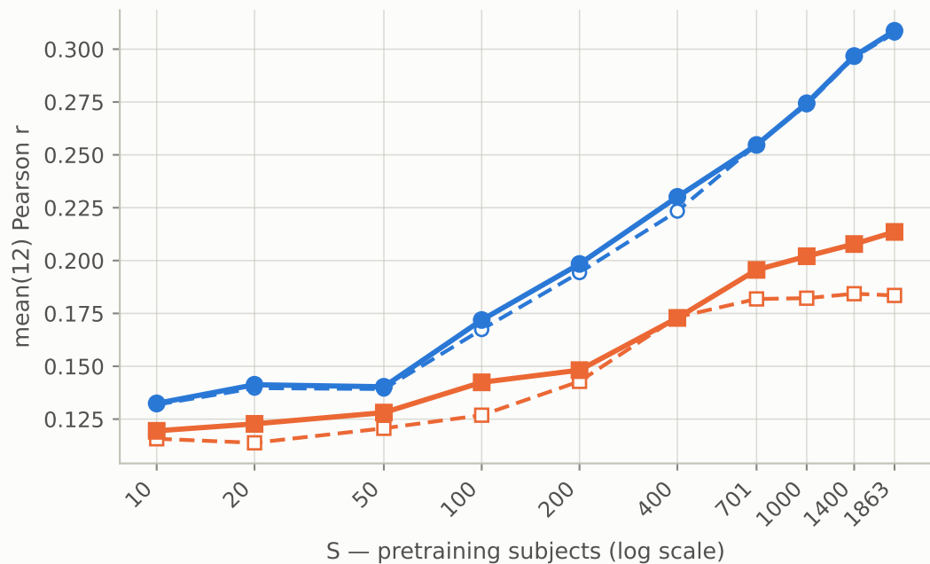
Within-task probe
