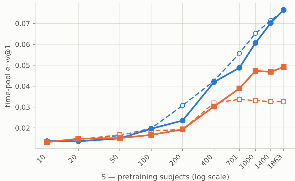
Within-task retrieval
