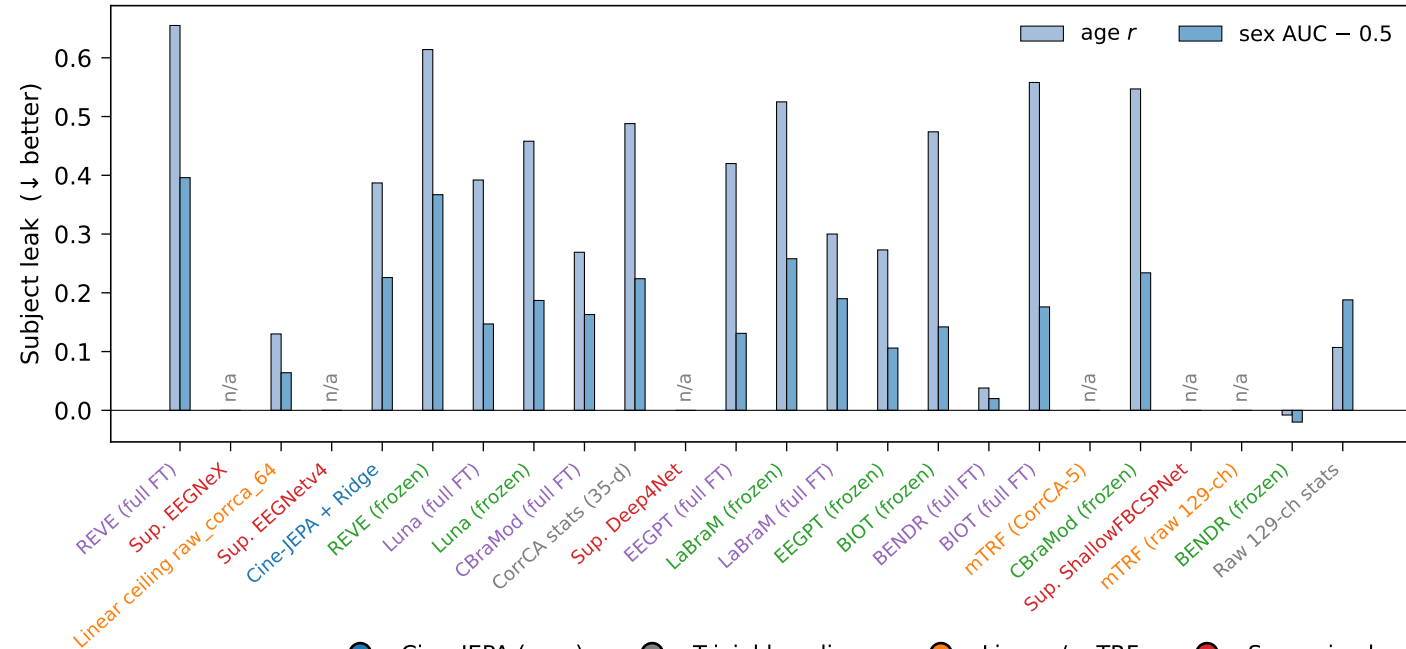
B. Subject anti-target (age r vs 0; sex AUC vs 0.5)
