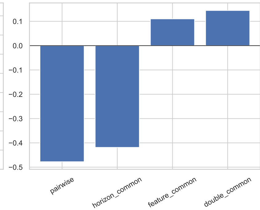
Mean distance-vs-Kendall rho
