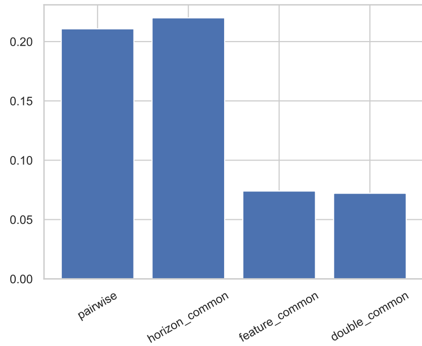
Mean |partial correlation|
