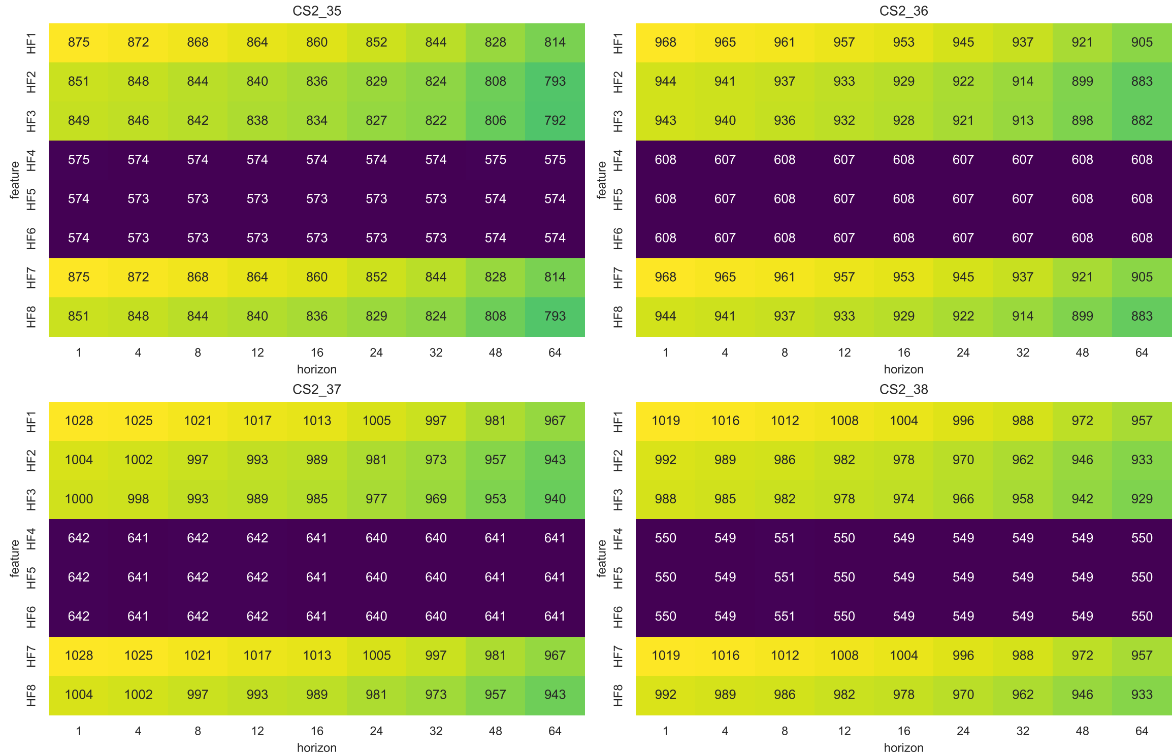
V2-1 Effective sample size under pairwise support
