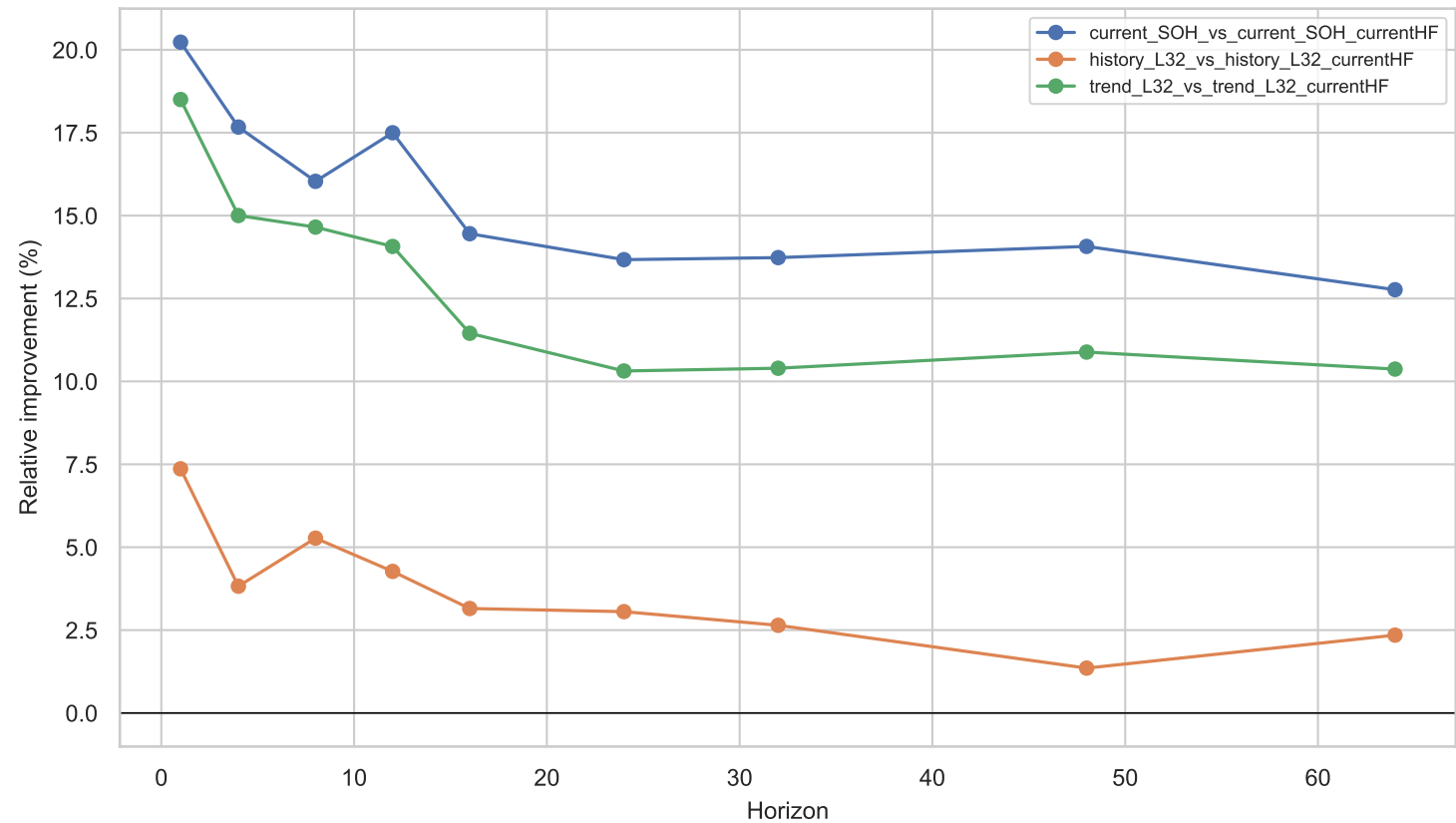
V2-7 Normalized prediction improvement
