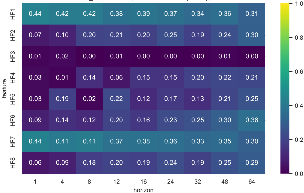
CS2_35: Absolute partial correlation | SOH(t)
