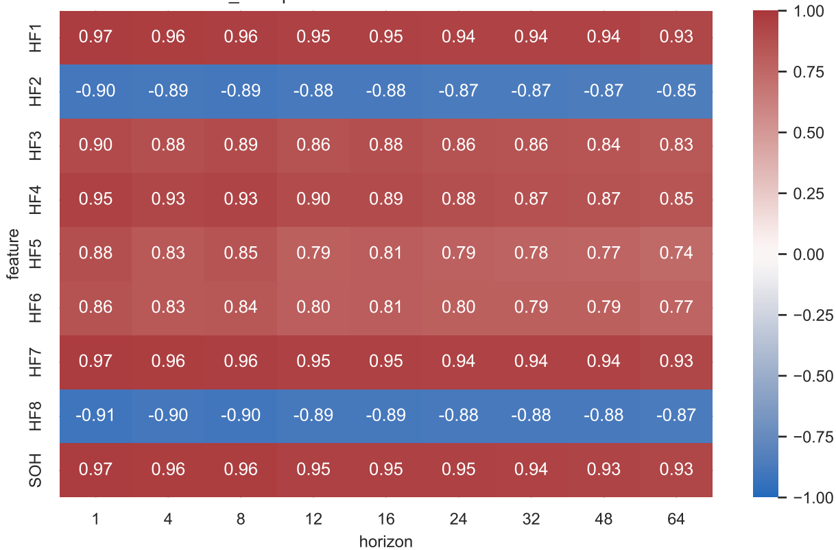
CS2_35: Spearman correlation with future SOH
