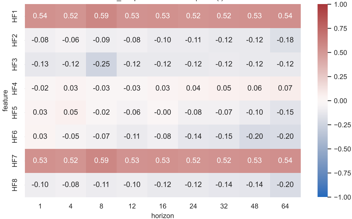
CS2_36: partial correlation | SOH(t)
