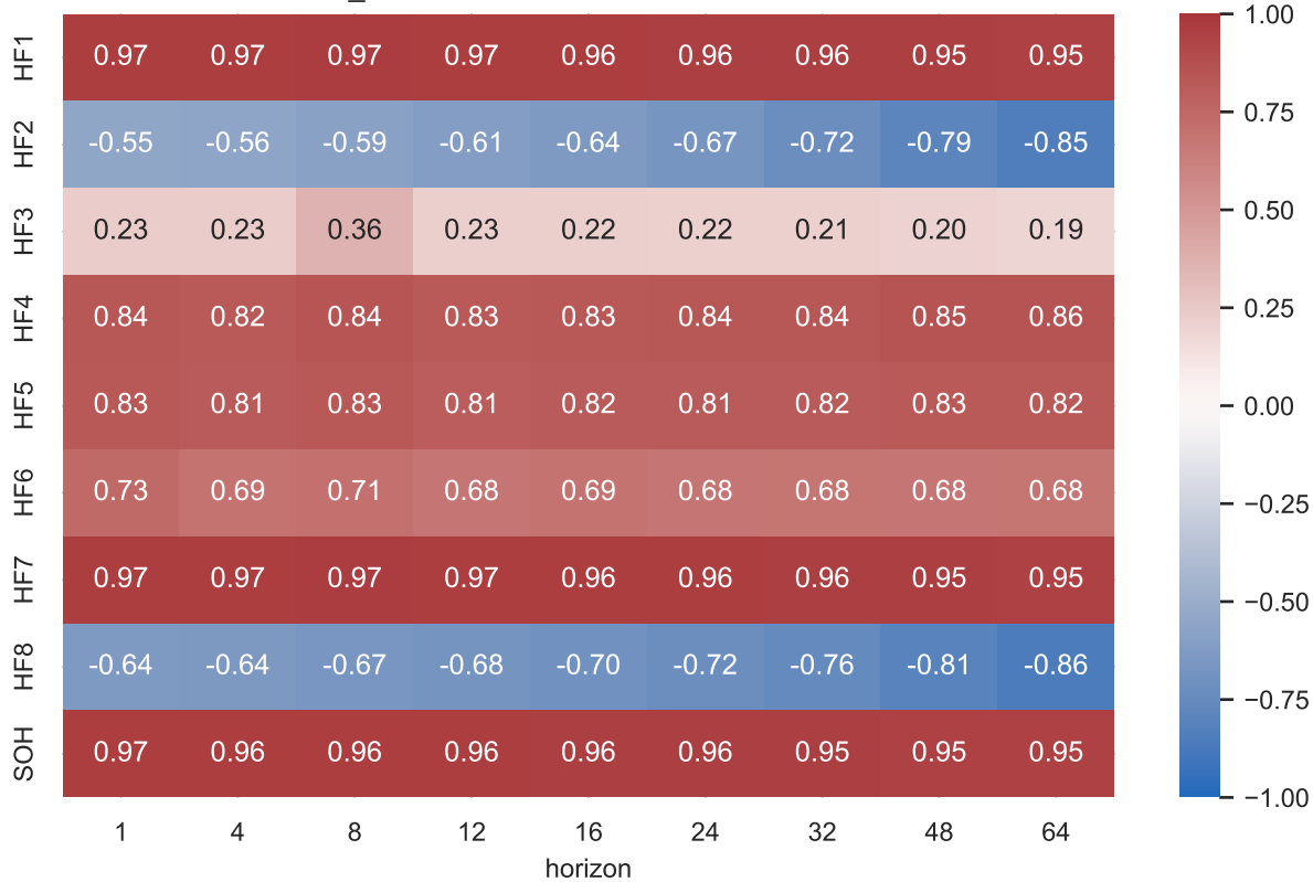
CS2_36: Pearson correlation with future SOH
